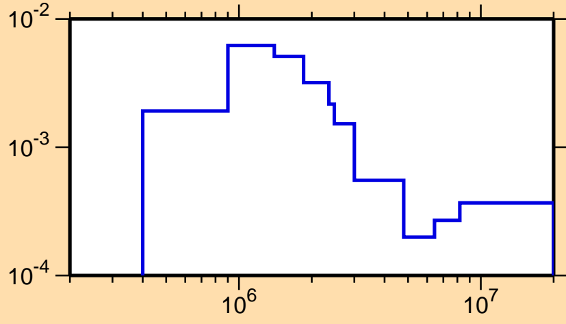
\sigma vs. E for ^{126}\text{La}(n,n_4)
