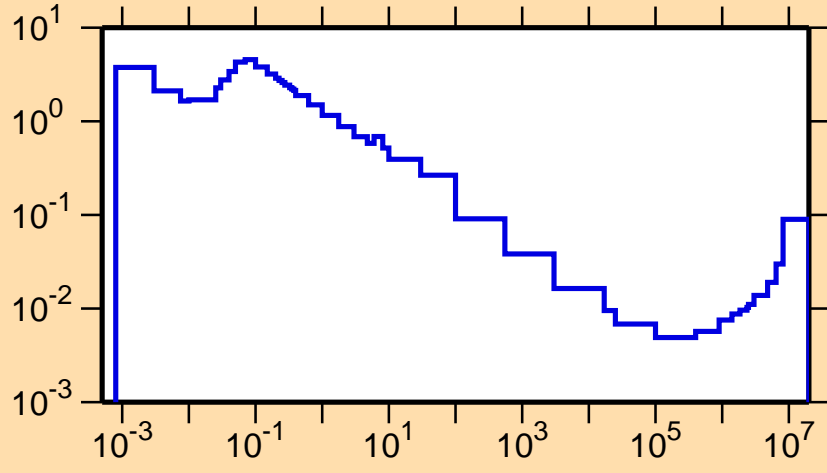
\sigma vs. E for ^{126}\text{La}(n,\alpha)
