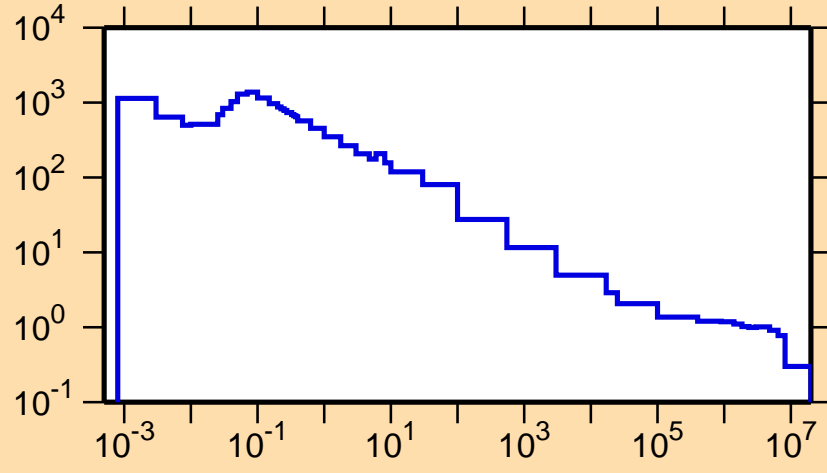
\sigma vs. E for ^{126}\text{La}(n,p)
