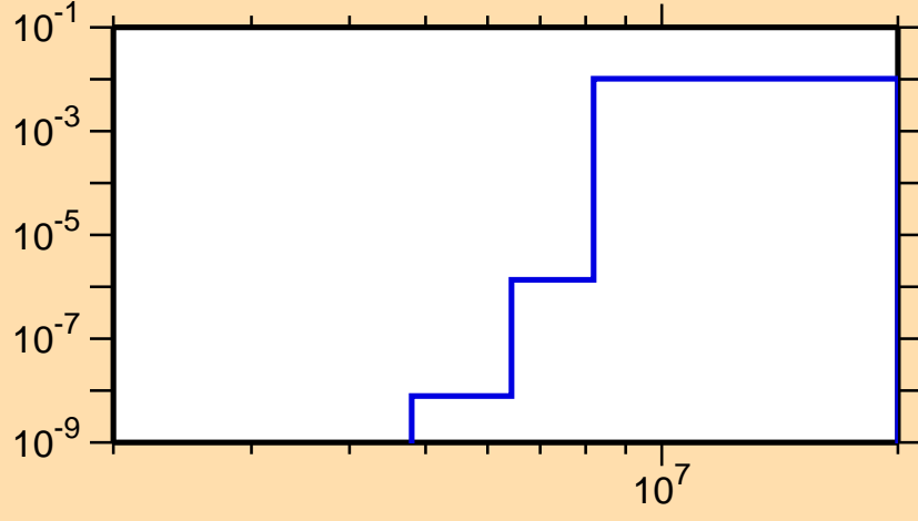
\sigma vs. E for ^{126}\text{La}(n,n\alpha)
