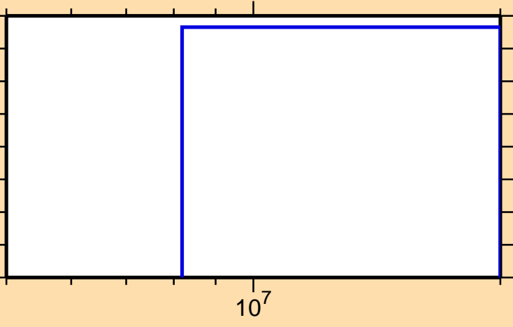
\sigma vs. E for ^{126}\text{La}(\text{mt117})
