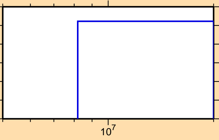
\sigma vs. E for ^{126}\text{La}(n,\text{nd})
