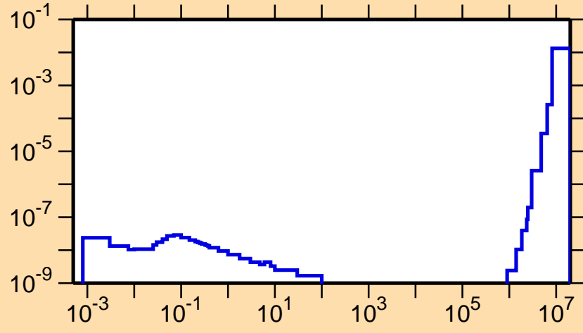
\sigma vs. E for ^{126}\text{La}(n,p\alpha)
