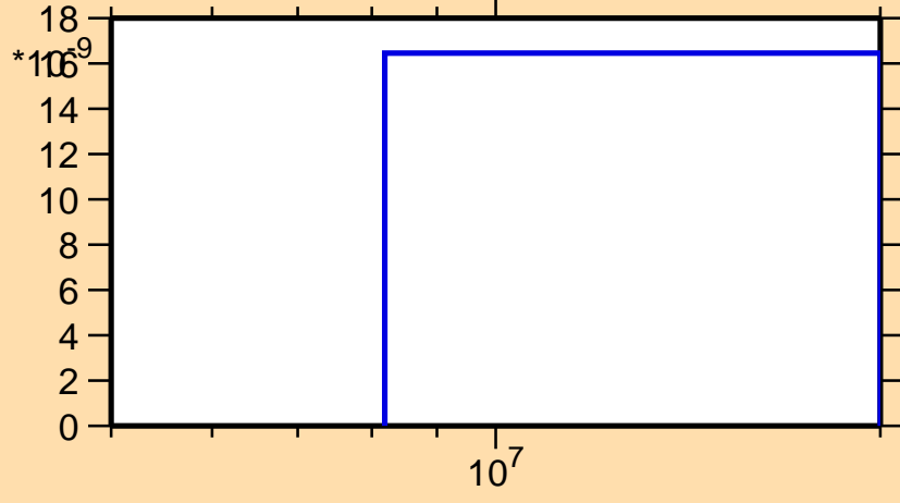
\sigma vs. E for ^{126}\text{La}(n,\text{pt})
