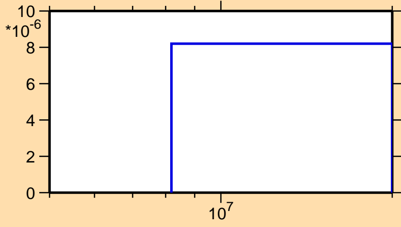
\sigma vs. E for ^{126}\text{La}(n,pd)
