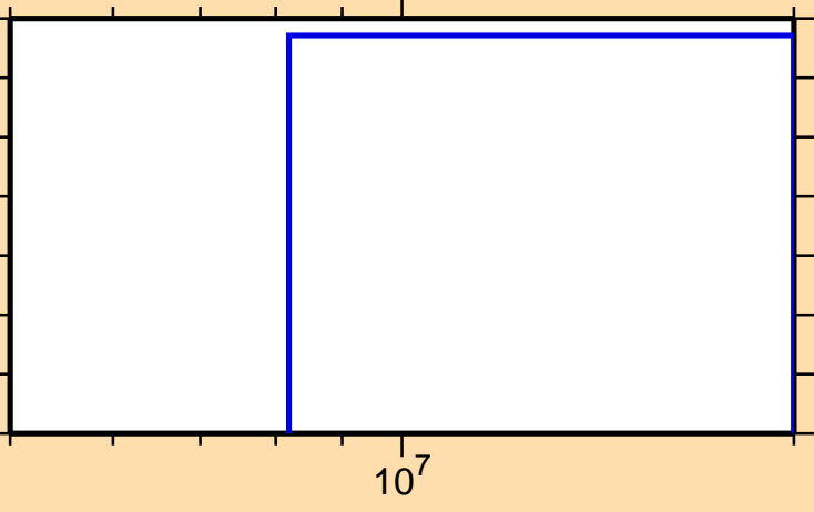
\sigma vs. E for ^{126}\text{La} (mt 45)
