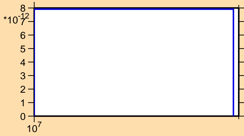
\sigma vs. E for ^{127}\text{La}(n,pt)
