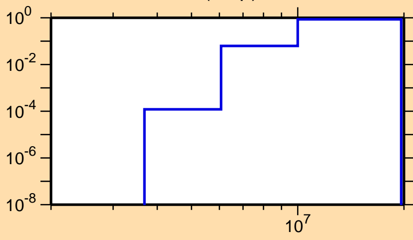
\sigma vs. E for ^{127}\text{La}(n,np)
