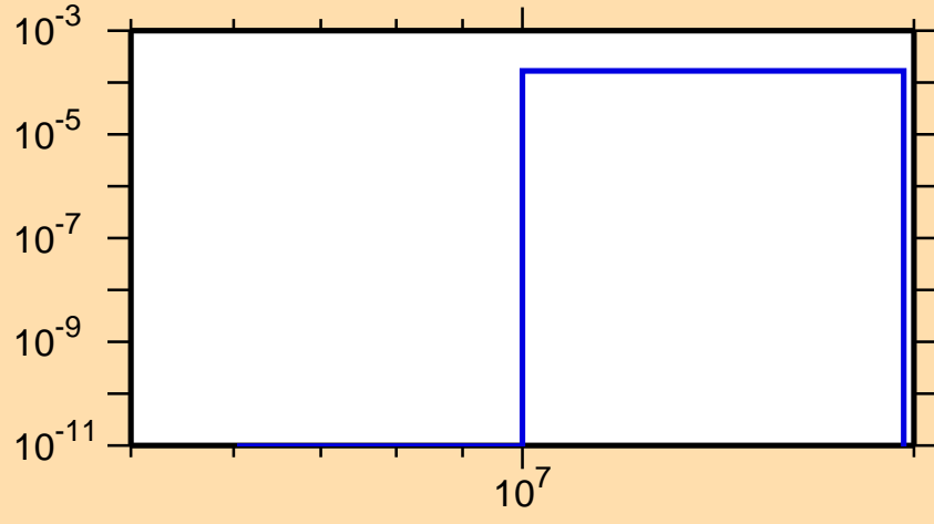
\sigma vs. E for ^{127}\text{La}(n,t)
