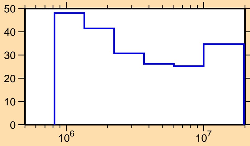
\Delta\sigma/\sigma vs. E for ^{127}\text{La}(n,ncont.)
