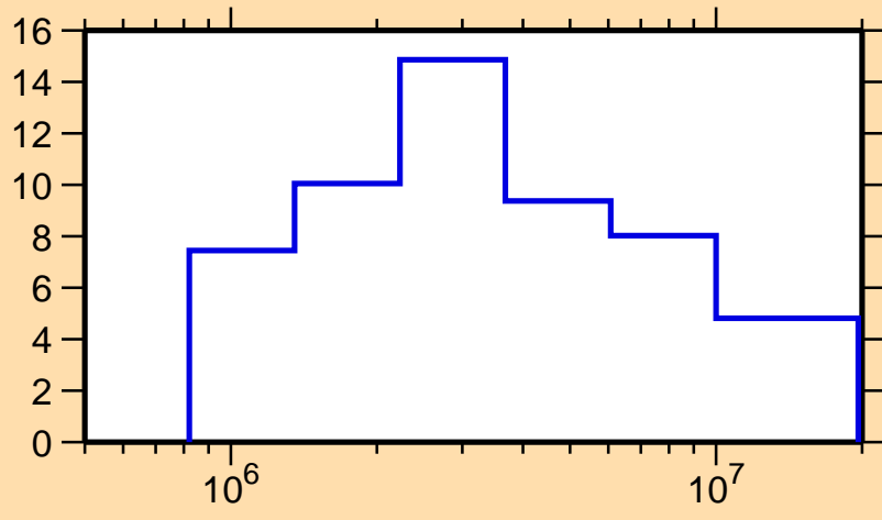
\Delta\sigma/\sigma vs. E for ^{127}\text{La}(n, el.)
