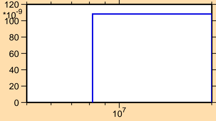
\sigma vs. E for ^{127}\text{La}(n,pd)
