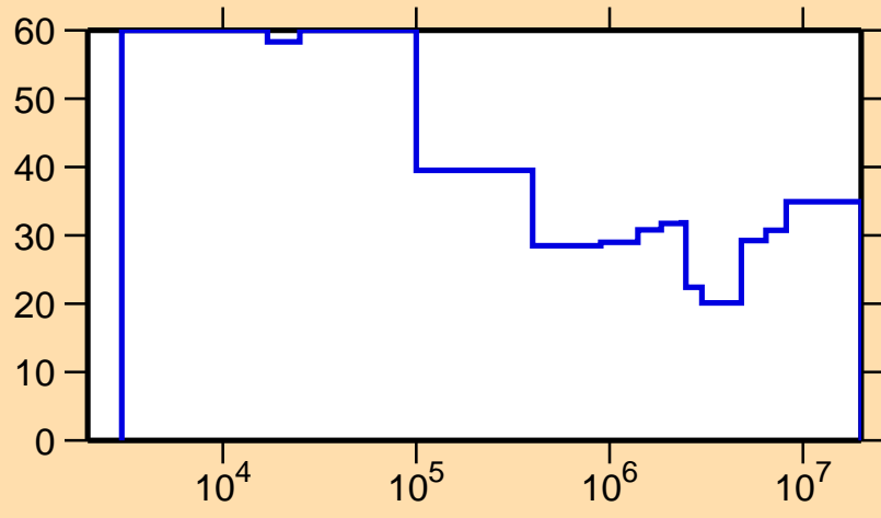
\Delta\sigma/\sigma vs. E for ^{127}\text{La}(n,n_1)
