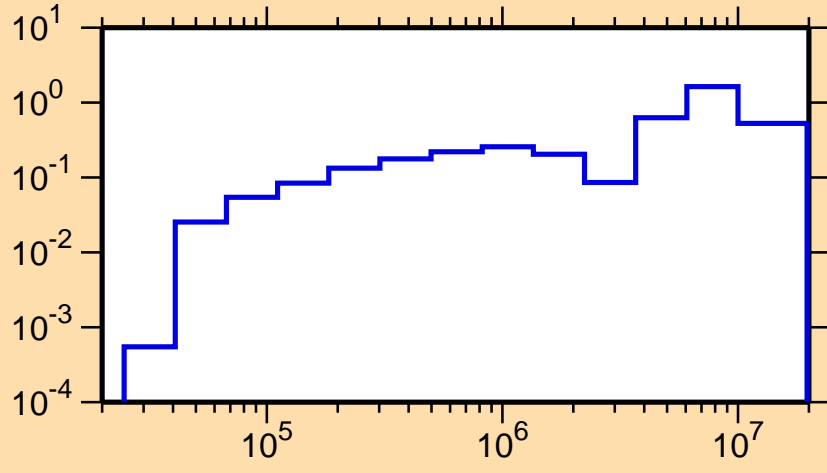
\sigma vs. E for ^{128}\text{La}(n,\text{inel.})
