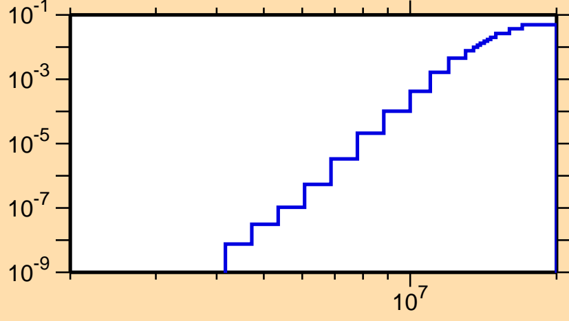
\sigma vs. E for ^{128}\text{La}(n,n\alpha)
