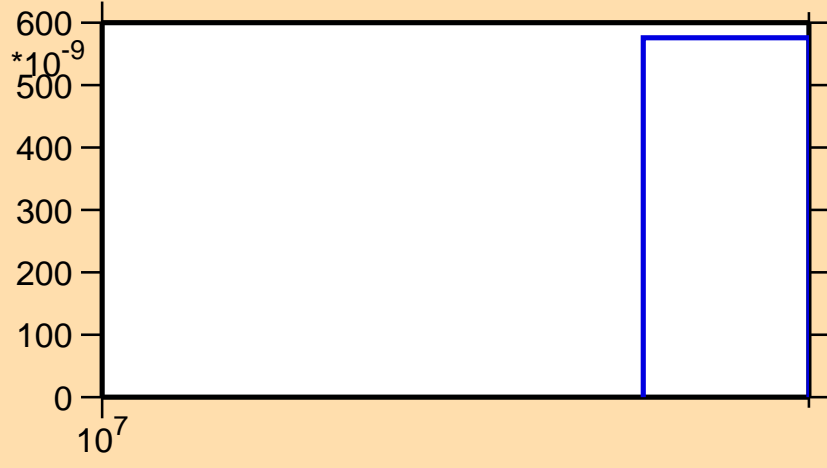
\sigma vs. E for ^{129}\text{La}(n,3n)
