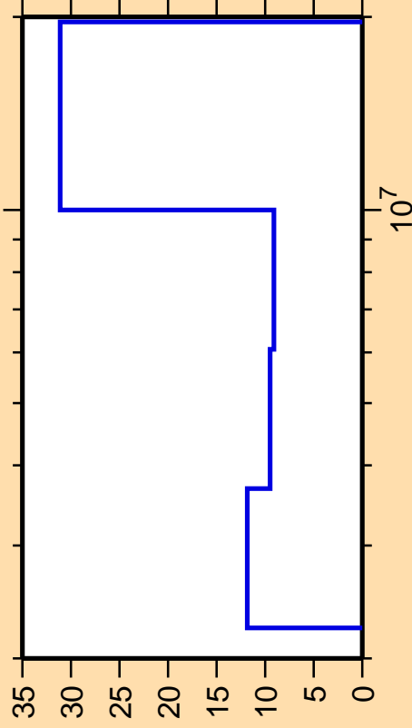
\Delta\sigma/\sigma vs. E for ^{129}\text{La}(n,\text{ncont.})
