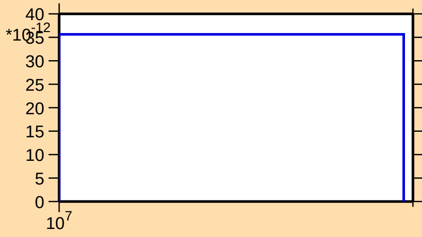
\sigma vs. E for ^{130}\text{La}(\text{mt117})
