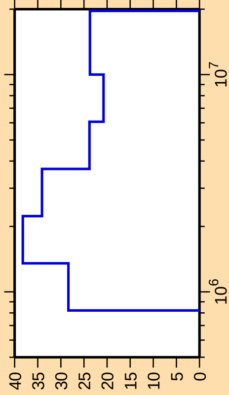
\Delta\sigma/\sigma vs. E for ^{130}\text{La}(n,p)
