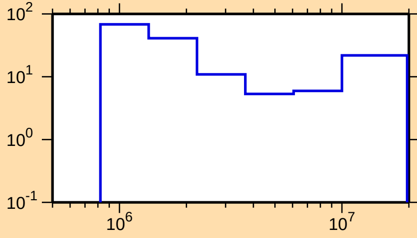
\Delta\sigma/\sigma vs. E for ^{130}\text{La}(n,n\text{cont.})
