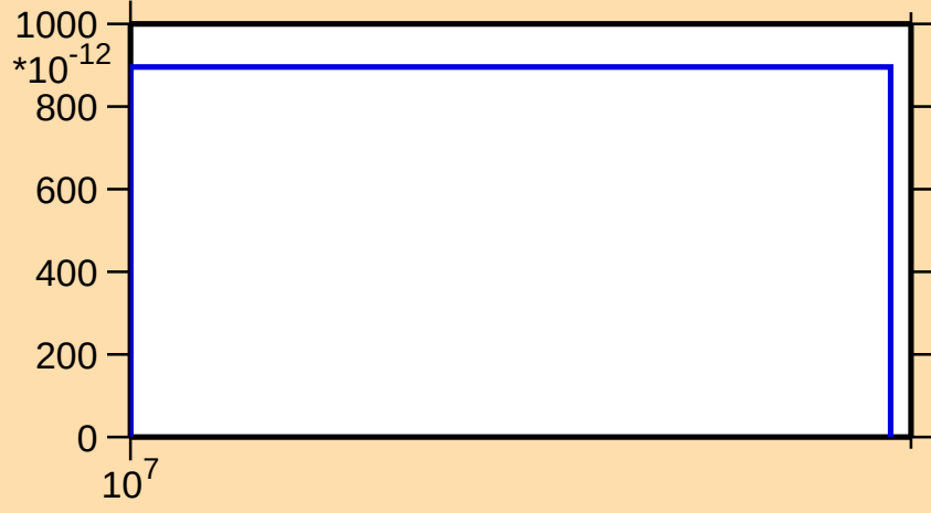
\sigma vs. E for ^{130}\text{La} (mt 45)
