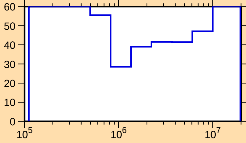
\Delta\sigma/\sigma vs. E for ^{130}\text{La}(n,n_1)
