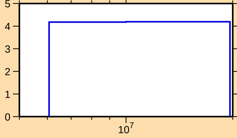
\Delta\sigma/\sigma vs. E for ^{130}\text{La}(n,\text{el.})
