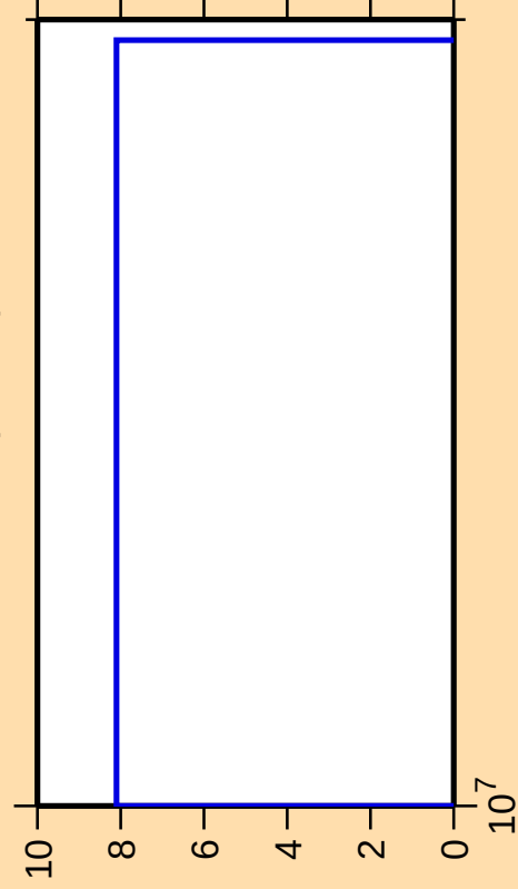
\Delta\sigma/\sigma vs. E for ^{130}\text{La} (mt 34)
