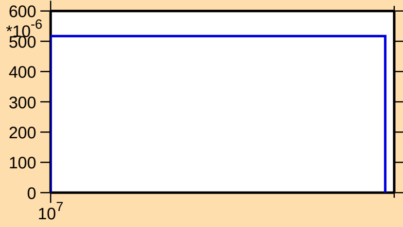
\sigma vs. E for ^{130}\text{La}(n,2np)
