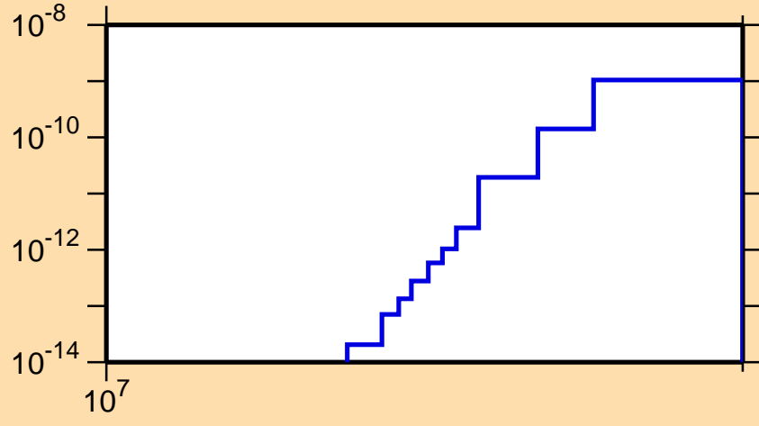
\sigma vs. E for ^{131}\text{La}(\text{mt117})
