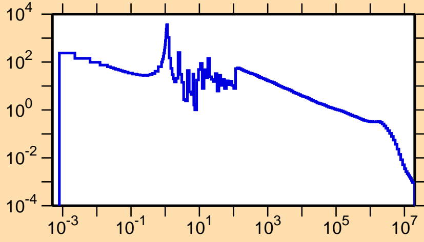
\sigma vs. E for ^{131}\text{La}(n,\gamma)
