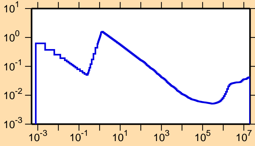
\sigma vs. E for ^{131}\text{La}(n,p)
