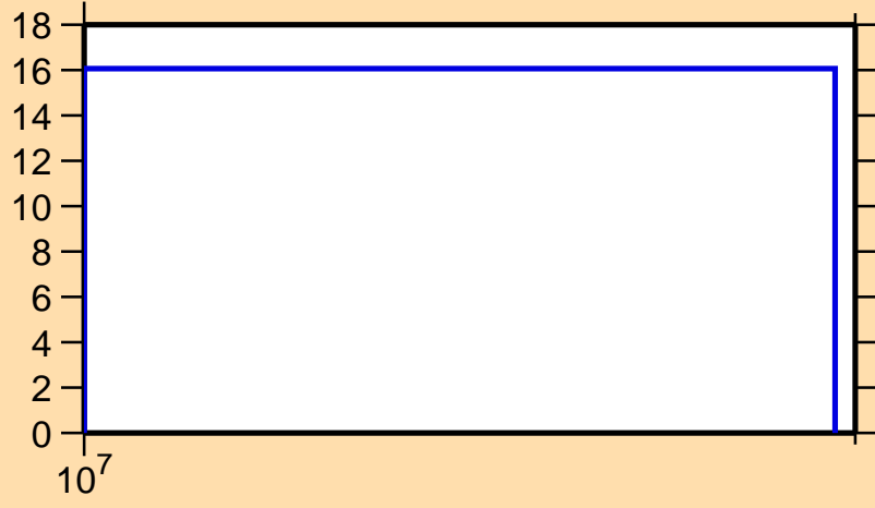
\Delta\sigma/\sigma vs. E for ^{131}\text{La}(n,\text{el.})
