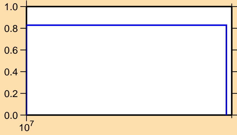
\sigma vs. E for ^{131}\text{La}(n,2n)
