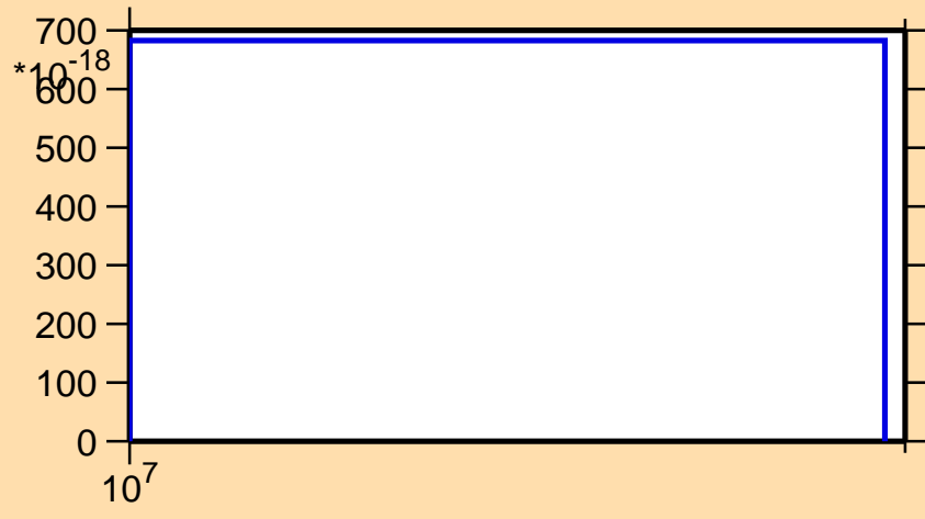
\sigma vs. E for ^{131}\text{La}(n,\text{pt})
