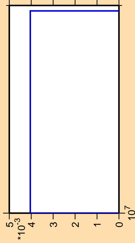
\Delta\sigma/\sigma vs. E for ^{131}\text{La} (mt 34)
