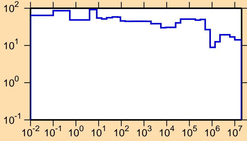
\Delta\sigma/\sigma vs. E for ^{131}\text{La}(n,\text{nonel.})
