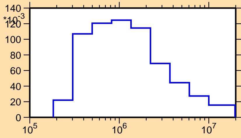
\sigma vs. E for ^{131}\text{La}(n,n_4)
