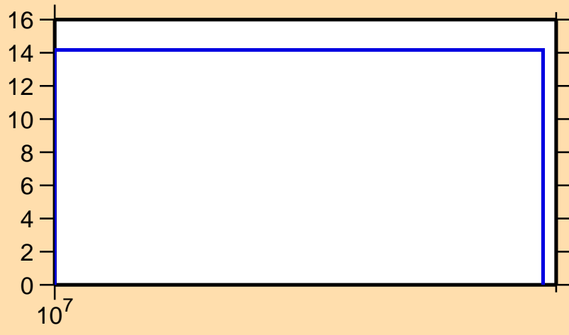
\Delta\sigma/\sigma vs. E for ^{131}\text{La}(n,\text{nonel.})
