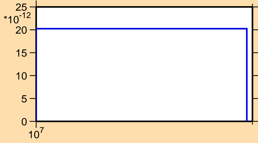
\sigma vs. E for ^{131}\text{La}(\text{mt117})
