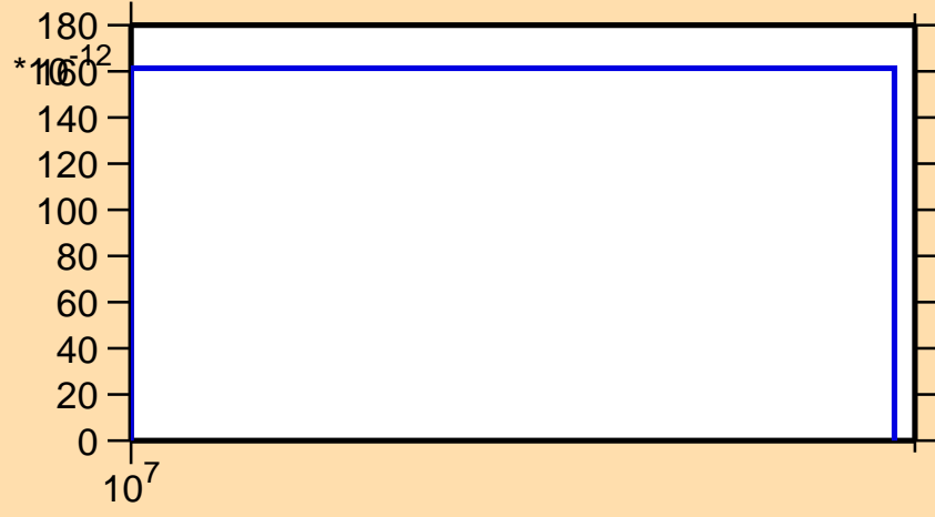
\sigma vs. E for ^{131}\text{La}(n,\text{pd})
