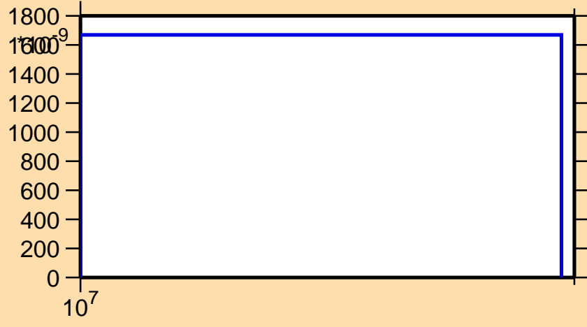
\sigma vs. E for ^{131}\text{La}(n,2np)
