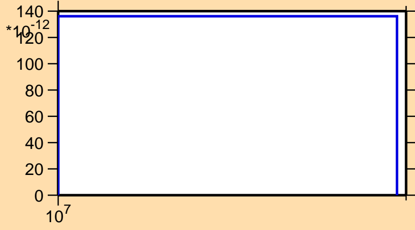
\sigma vs. E for ^{131}\text{La}(n,2n\alpha)
