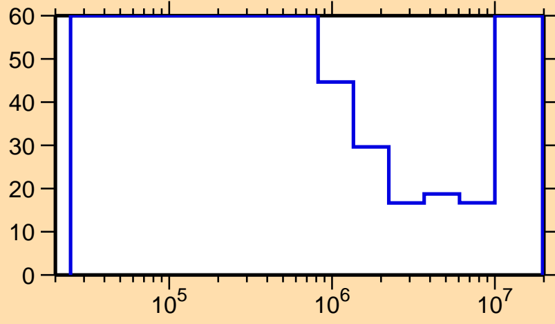
\Delta\sigma/\sigma vs. E for ^{131}\text{La}(n,\text{inel.})
