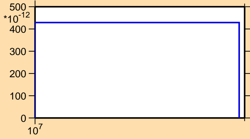
\sigma vs. E for ^{131}\text{La}(n,nt)
