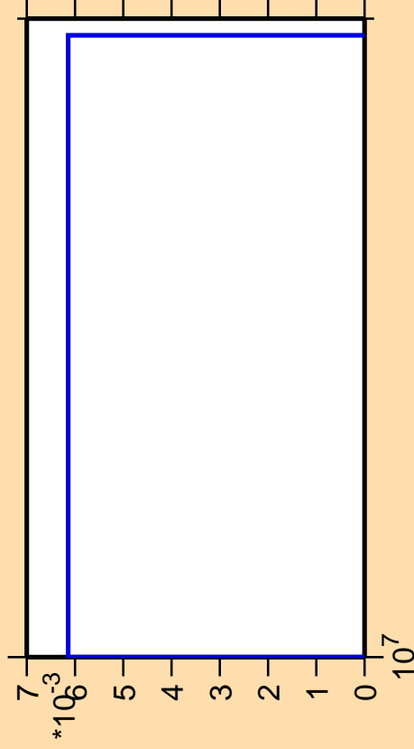
\Delta\sigma/\sigma vs. E for ^{131}\text{La}(n,\text{pt})
