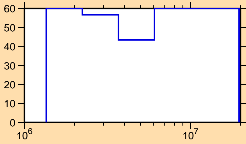
\Delta\sigma/\sigma vs. E for ^{131}\text{La}(n,n_1)
