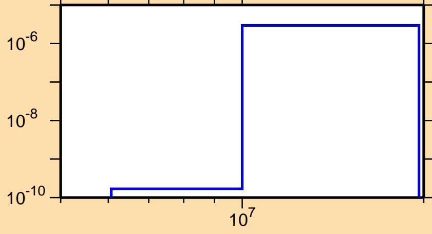
\sigma vs. E for ^{131}\text{La}(n,p\alpha)
