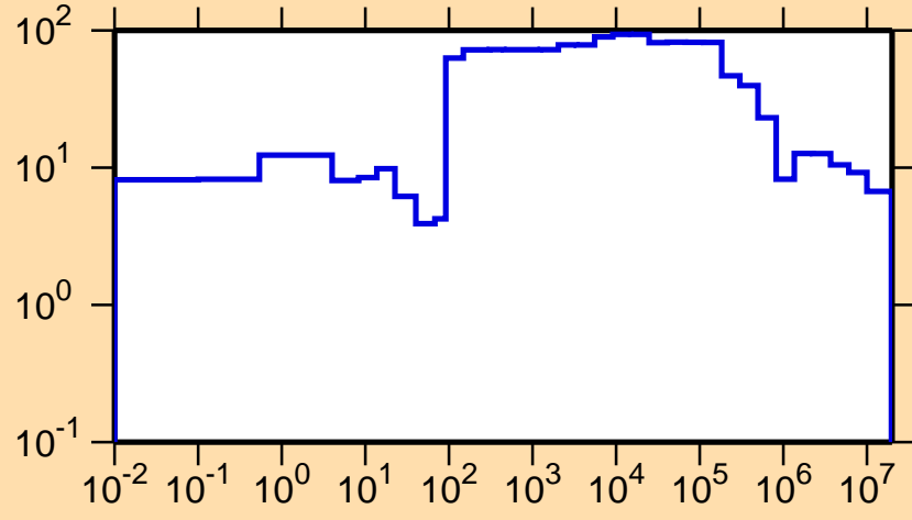
\Delta\sigma/\sigma vs. E for ^{131}\text{La}(n,\text{tot.})
