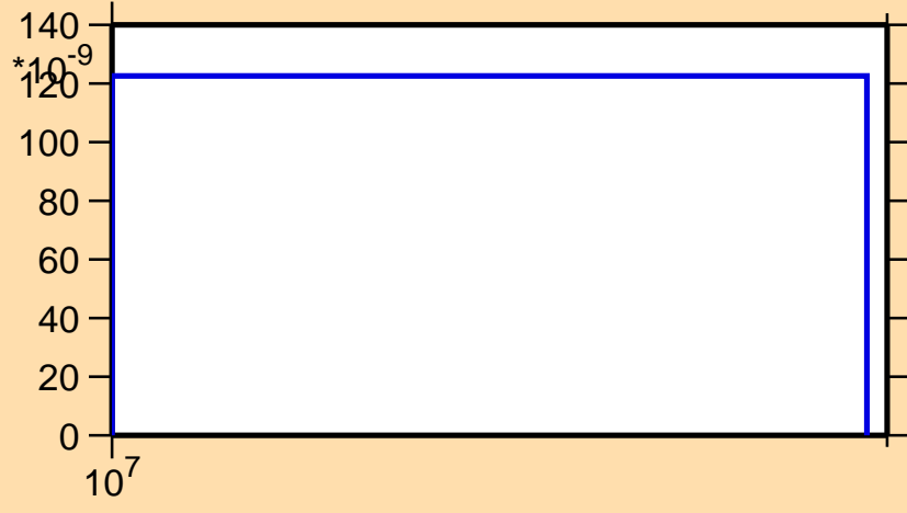
\sigma vs. E for ^{131}\text{La}(n,\text{nd})
