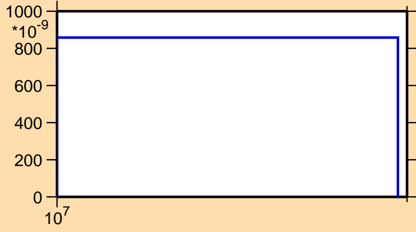
\sigma vs. E for ^{131}\text{La}(n,3n)
