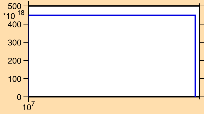
\sigma vs. E for ^{131}\text{La} (mt 34)
