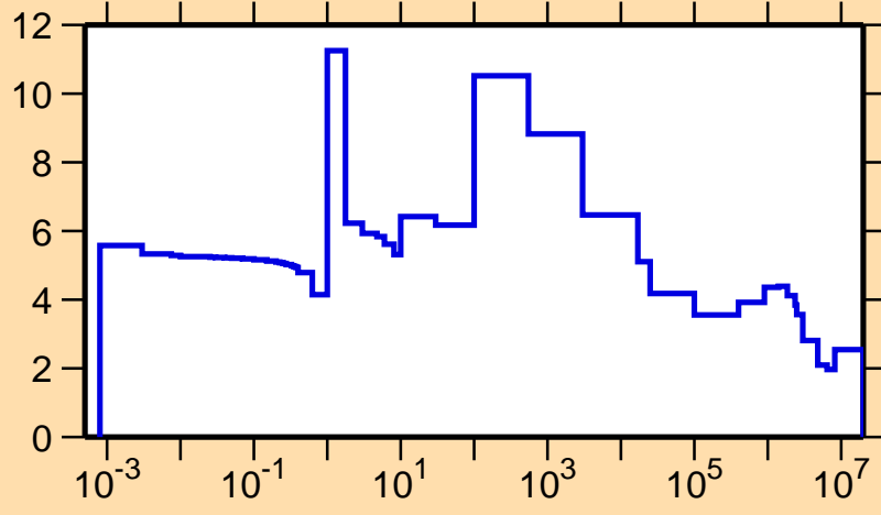
\sigma vs. E for ^{131}\text{La}(n,\text{el.})
