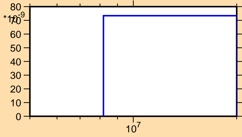
\sigma vs. E for ^{131}\text{La}(n,\text{He3})
