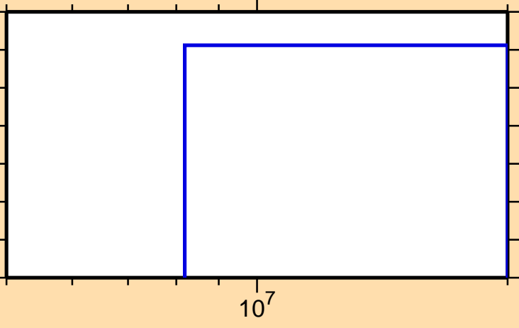
\sigma vs. E for ^{131}\text{La} (mt 34)
