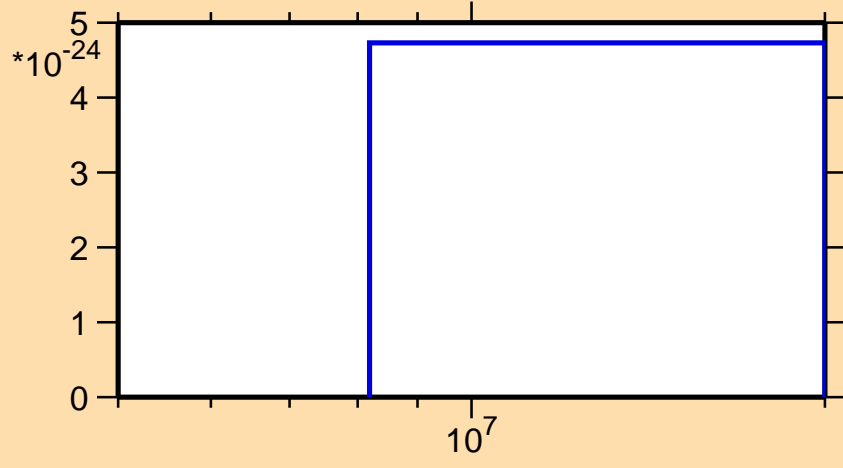
\sigma vs. E for ^{131}\text{La} (mt 11)
