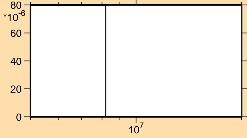
\sigma vs. E for ^{131}\text{La}(n,t)
