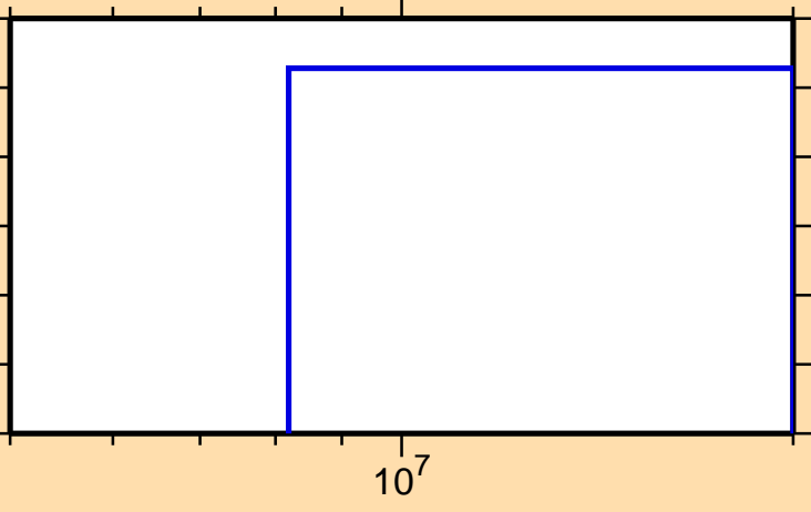
\sigma vs. E for ^{131}\text{La}(n,\text{nd})
