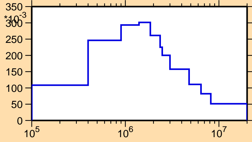
\sigma vs. E for ^{131}\text{La}(n,n_2)
