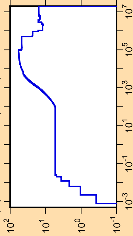
\Delta\mu/\mu vs. E for ^{132}\text{La}(\text{mt251})
