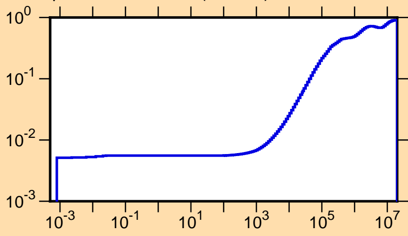
\mu vs. E for ^{132}\text{La}(\text{mt251})
