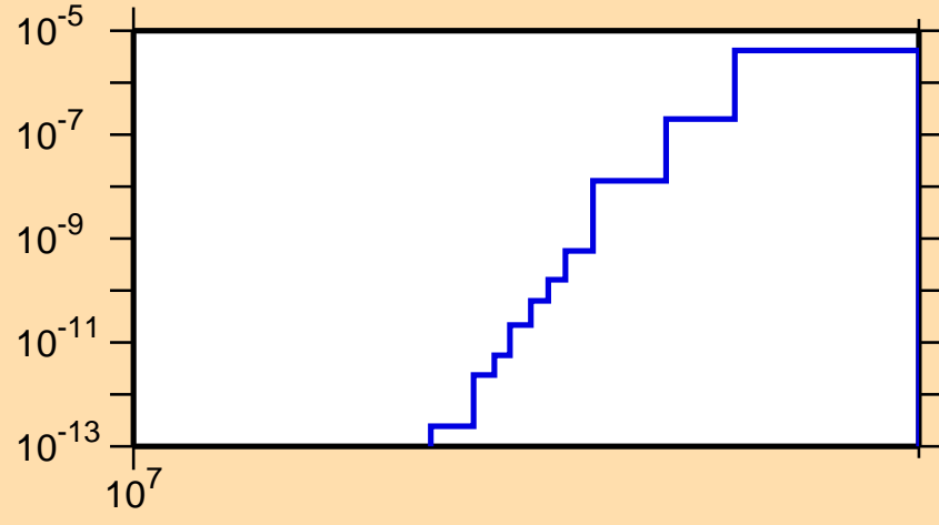
\sigma vs. E for ^{132}\text{La}(n,2n\alpha)
