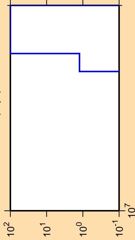
\Delta\sigma/\sigma vs. E for ^{132}\text{La}(n,pt)
