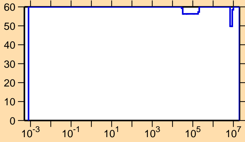
\Delta\sigma/\sigma vs. E for ^{132}\text{La}(n,p)
