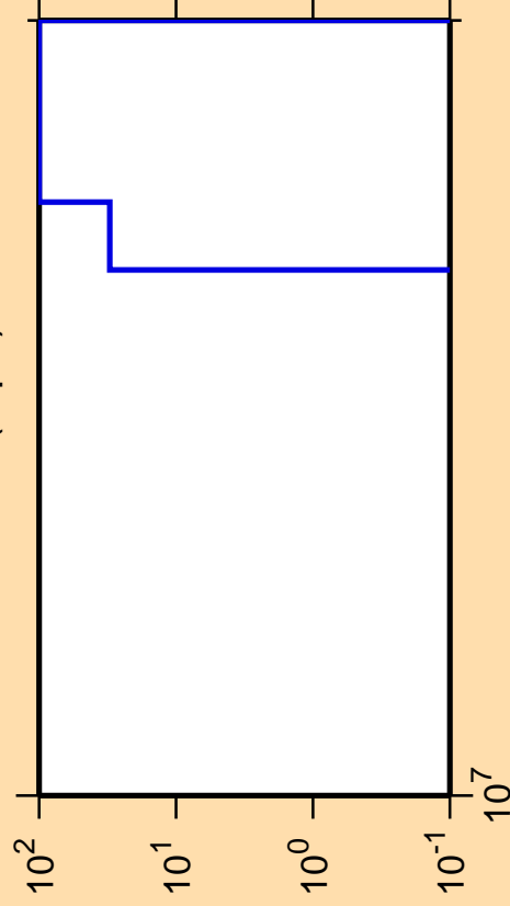
\Delta\sigma/\sigma vs. E for ^{132}\text{La}(n,\text{pd})
