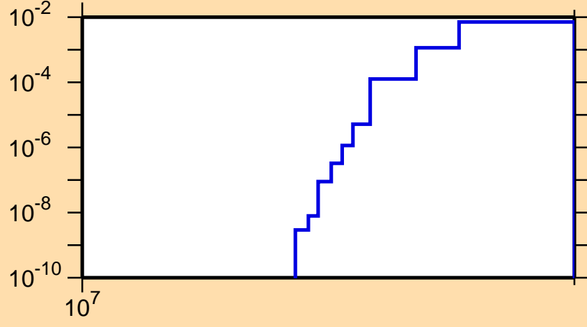
\sigma vs. E for ^{132}\text{La}(n,2np)
