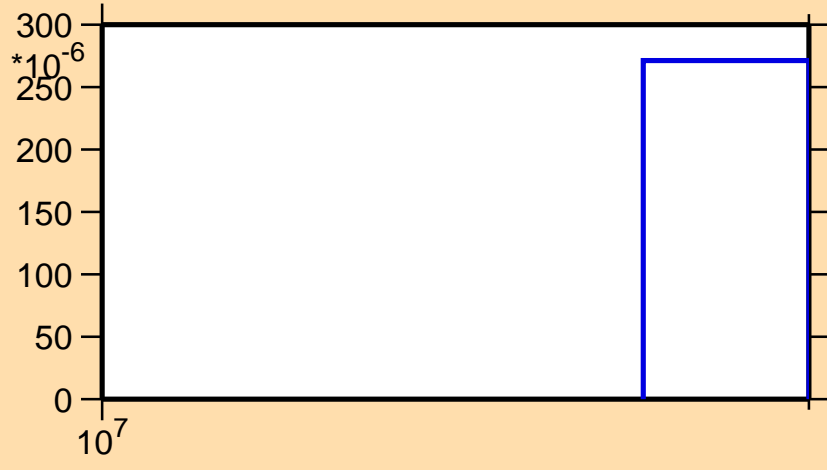
\sigma vs. E for ^{132}\text{La}(n,3n)
