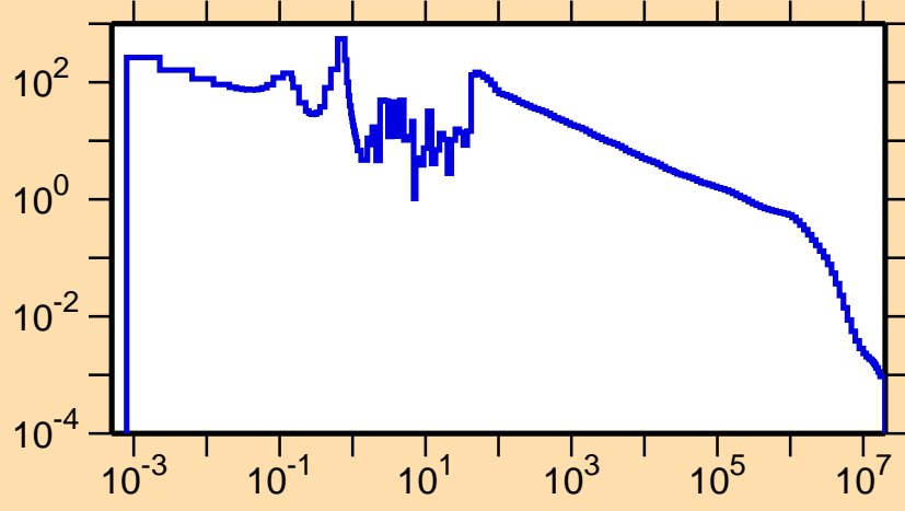
\sigma vs. E for ^{132}\text{La}(n,\gamma)
