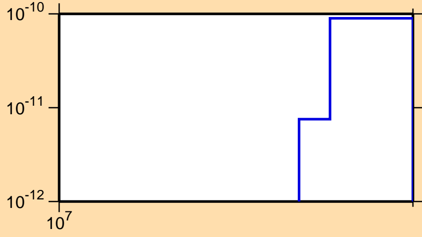
\sigma vs. E for ^{132}\text{La} (mt117)
