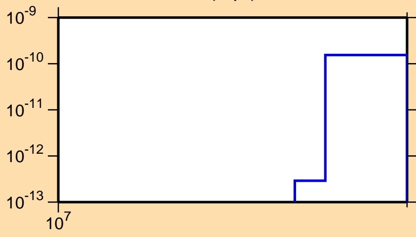
\sigma vs. E for ^{132}\text{La}(n,pt)
