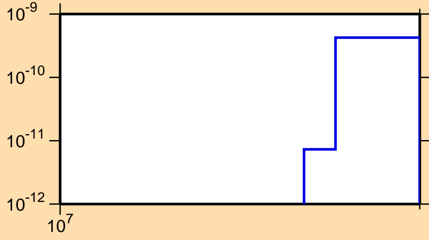
\sigma vs. E for ^{132}\text{La}(n,\text{pd})
