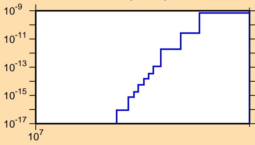
\sigma vs. E for ^{132}\text{La} (mt 45)
