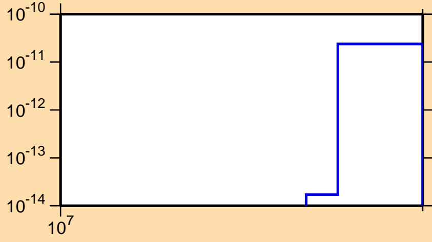
\sigma vs. E for ^{132}\text{La} (mt 34)
