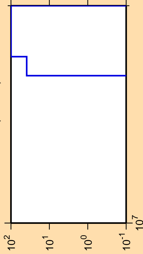
\Delta\sigma/\sigma vs. E for ^{132}\text{La} (mt117)
