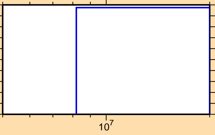
\sigma vs. E for ^{132}\text{La} (mt 34)
