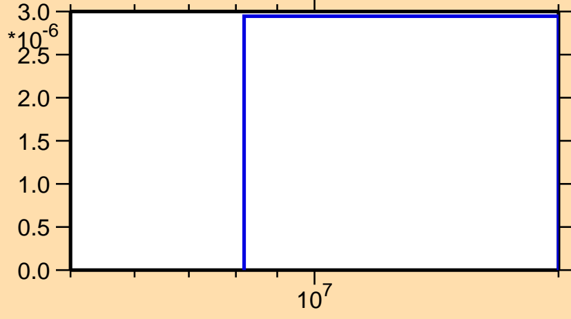
\sigma vs. E for ^{132}\text{La}(n,\text{nd})
