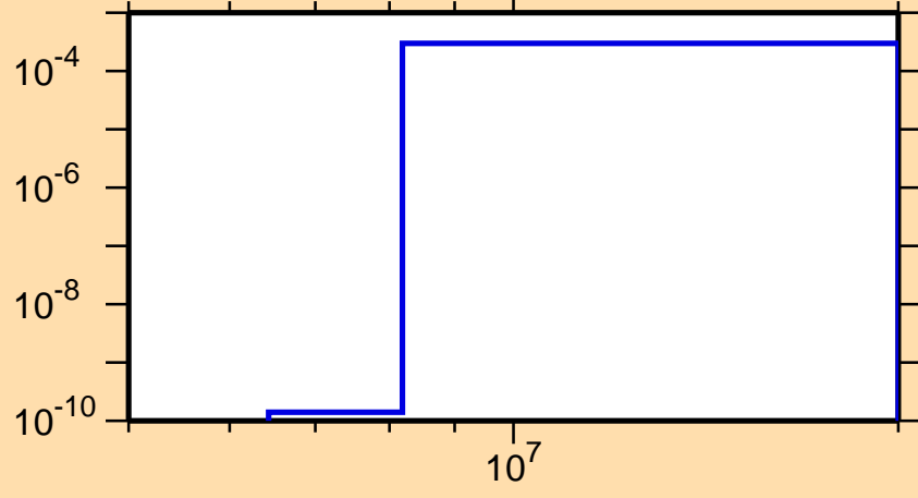
\sigma vs. E for ^{132}\text{La}(n,t)
