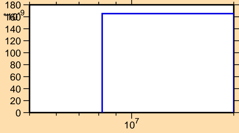
\sigma vs. E for ^{132}\text{La}(n,\text{He}3)
