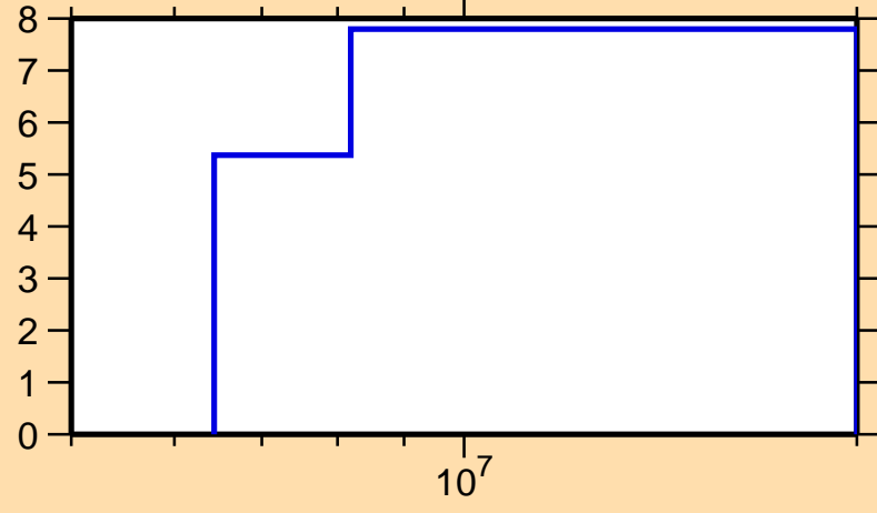
\Delta\sigma/\sigma vs. E for ^{132}\text{La}(n,\text{tot.})
