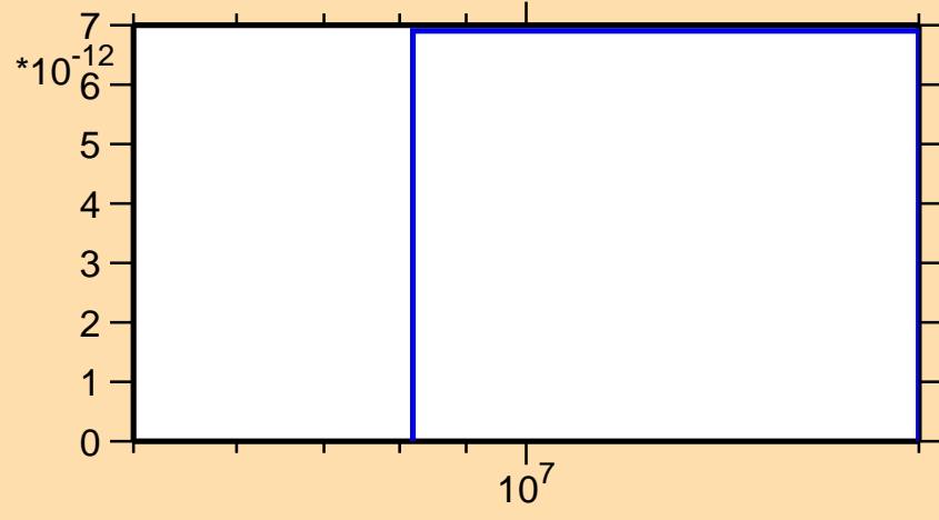
\sigma vs. E for ^{132}\text{La} (mt 45)
