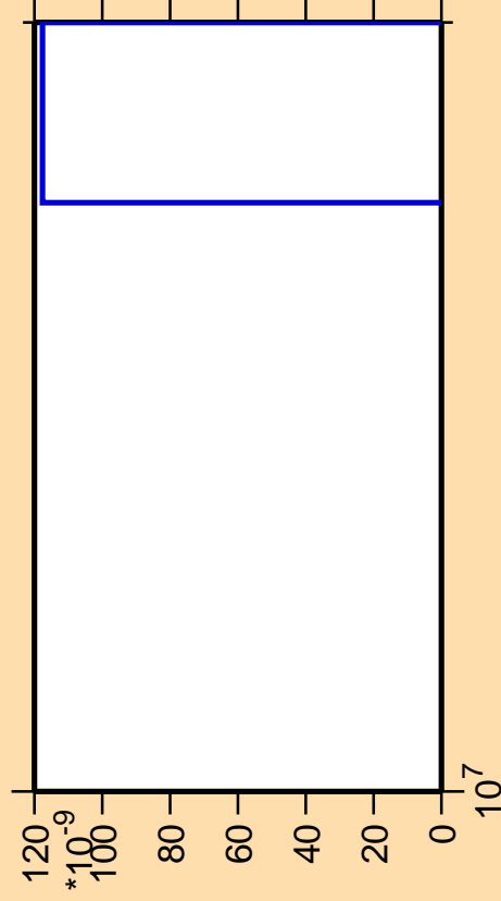
\Delta\sigma/\sigma vs. E for ^{132}\text{La} (mt 11)
