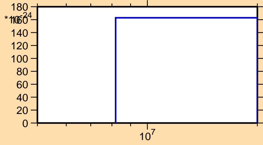
\sigma vs. E for ^{132}\text{La} (mt 11)
