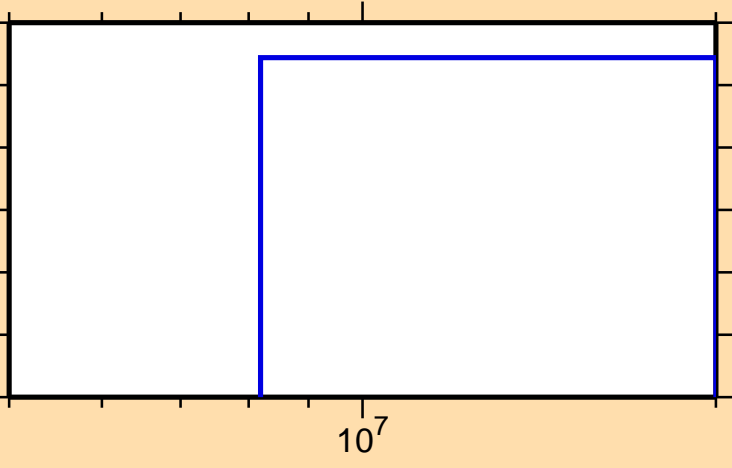
\sigma vs. E for ^{132}\text{La}(n,2np)
