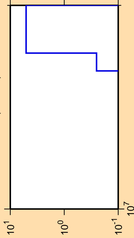
\Delta\sigma/\sigma vs. E for ^{134}\text{La}(\text{mt117})
