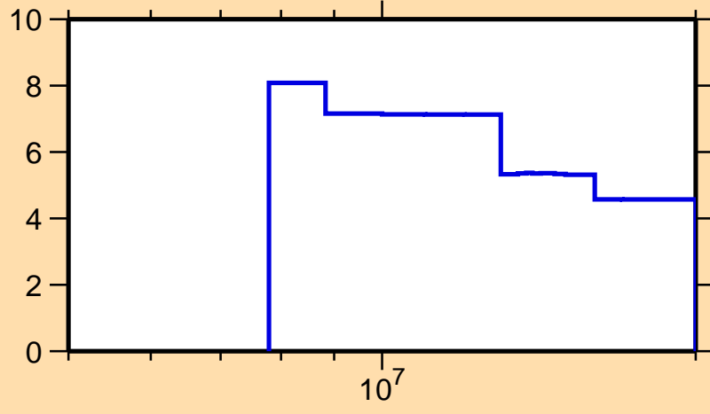
\Delta\sigma/\sigma vs. E for ^{134}\text{La}(n,2n)
