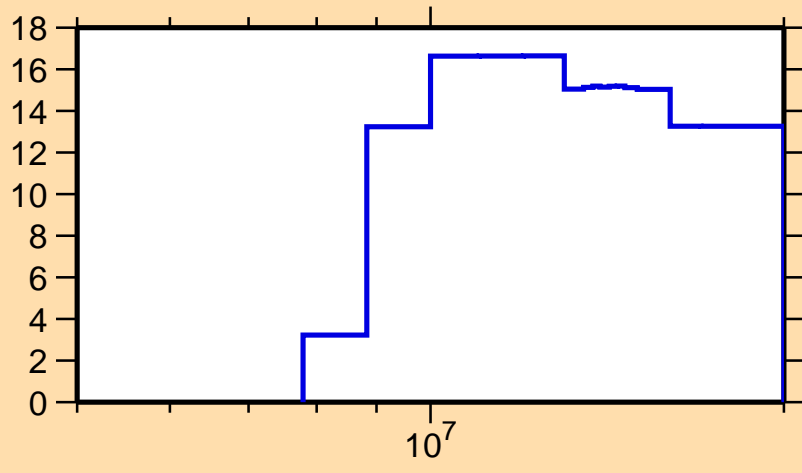
\Delta\sigma/\sigma vs. E for ^{134}\text{La}(n,\text{inel.})
