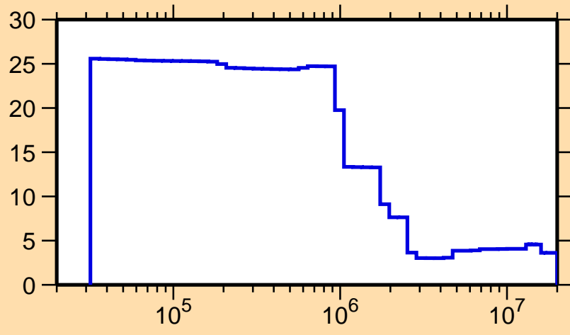
\Delta\sigma/\sigma vs. E for ^{134}\text{La}(n,\text{nonel.})
