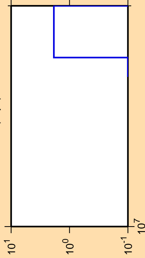
\Delta\sigma/\sigma vs. E for ^{134}\text{La}(n,\text{pt})
