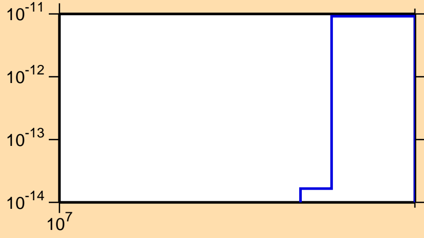
\sigma vs. E for ^{134}\text{La}(n,pd)
