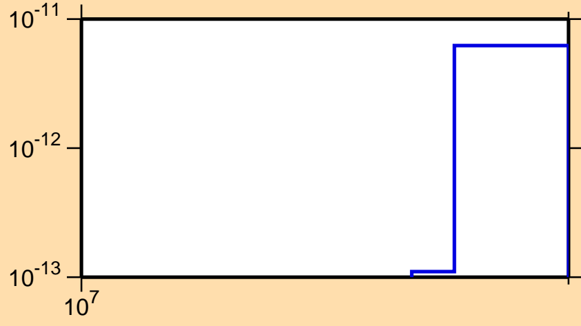
\sigma vs. E for ^{134}\text{La} (mt 45)
