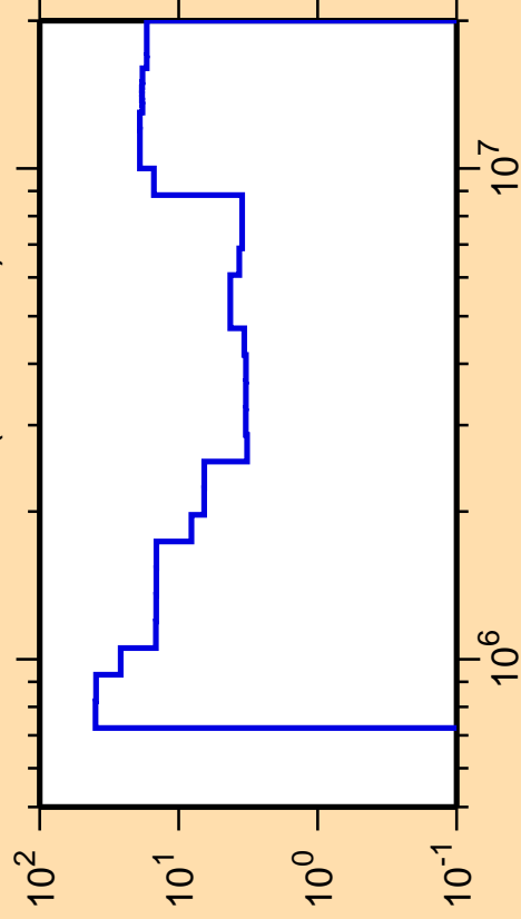
\Delta\sigma/\sigma vs. E for ^{134}\text{La}(n,\text{ncont.})
