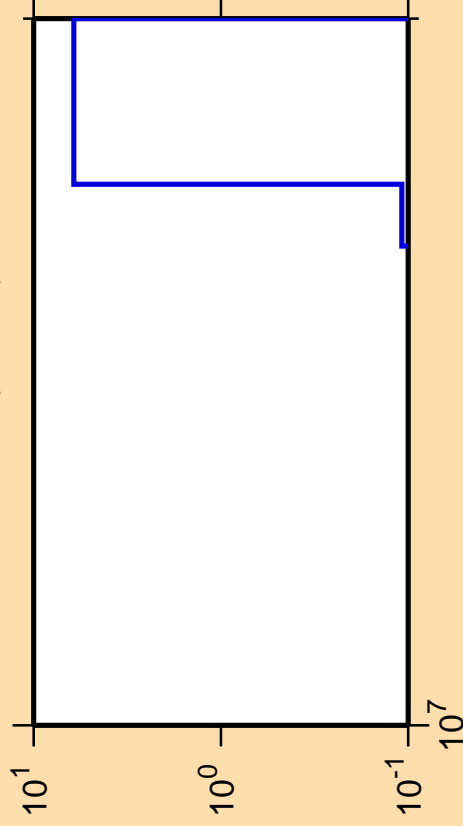
\Delta\sigma/\sigma vs. E for ^{134}\text{La} (mt 45)
