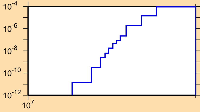
\sigma vs. E for ^{134}\text{La}(n,\text{nd})
