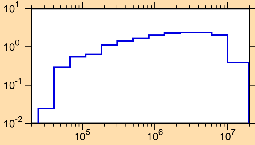
\sigma vs. E for ^{134}\text{La}(n,\text{inel.})
