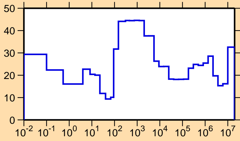
\Delta\sigma/\sigma vs. E for ^{134}\text{La}(n,\gamma)
