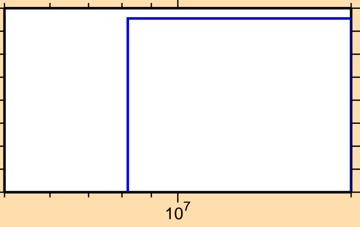
\sigma vs. E for ^{134}\text{La}(n,pd)
