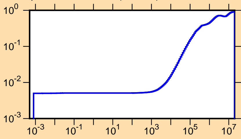
\mu vs. E for ^{135}\text{La}(\text{mt251})
