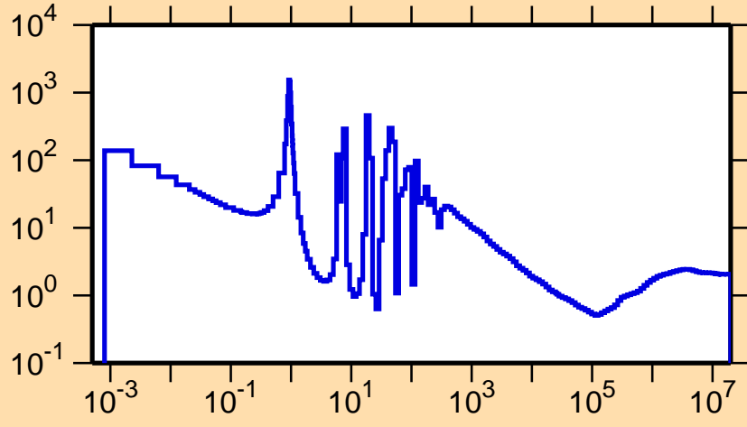
\sigma vs. E for ^{135}\text{La}(n,\text{nonel.})
