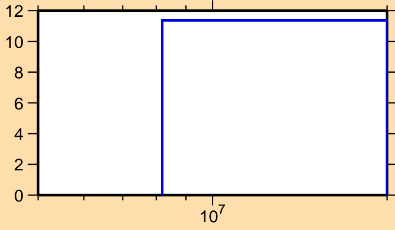
\Delta\sigma/\sigma vs. E for ^{135}\text{La}(n,2n)
