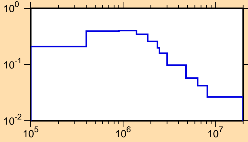
\sigma vs. E for ^{135}\text{La}(n,n_1)
