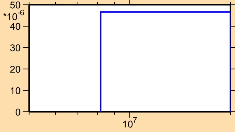
\sigma vs. E for ^{135}\text{La}(n,t)
