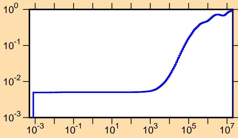
\mu vs. E for ^{136}\text{La}(\text{mt251})
