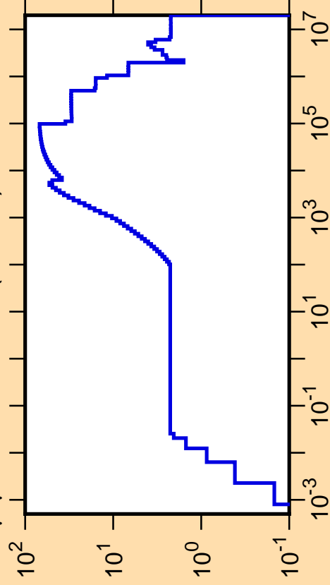
\Delta\mu/\mu vs. E for ^{136}\text{La}(\text{mt251})
