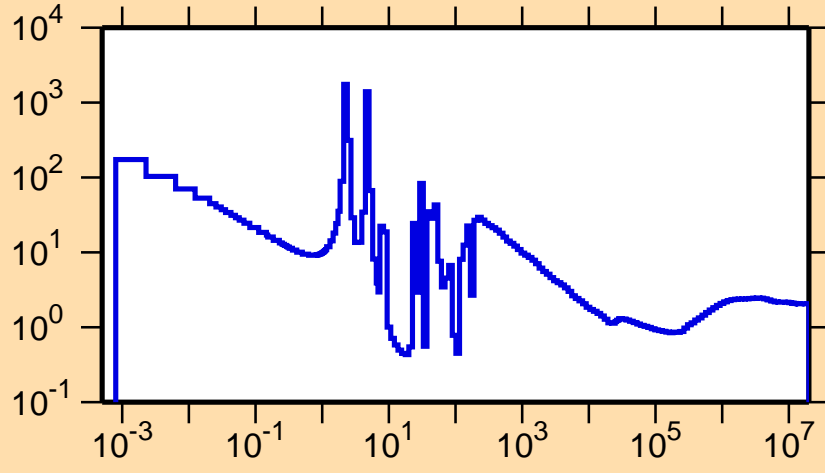
\sigma vs. E for ^{136}\text{La}(n,\text{nonel.})
