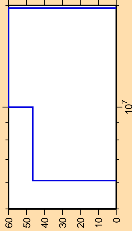
\Delta\sigma/\sigma vs. E for ^{136}\text{La}(n,n\alpha)
