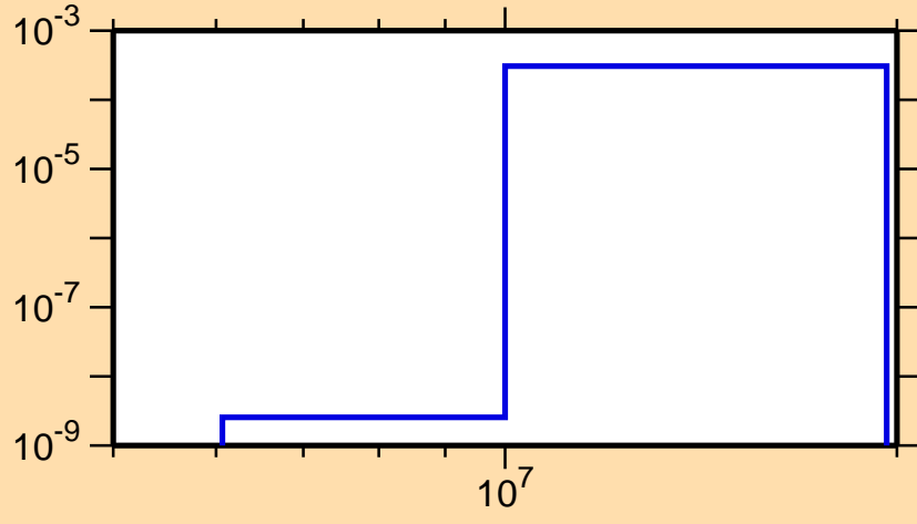
\sigma vs. E for ^{136}\text{La}(n,n\alpha)
