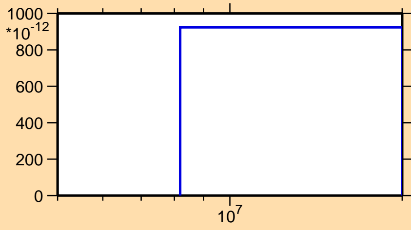
\sigma vs. E for ^{136}\text{La}(n,nt)
