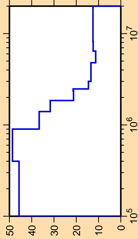
\Delta\sigma/\sigma vs. E for ^{136}\text{La}(n,n_3)
