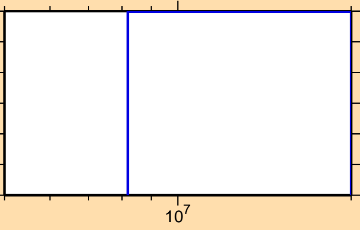
\sigma vs. E for ^{136}\text{La}(n,\text{He3})
