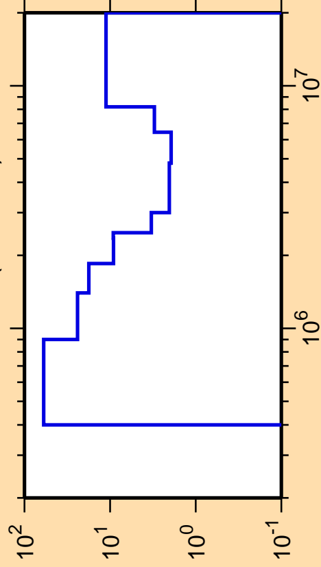
\Delta\sigma/\sigma vs. E for ^{136}\text{La}(n,\text{ncont.})
