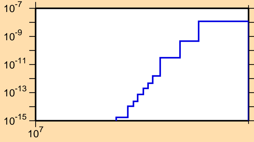
\sigma vs. E for ^{137}\text{La}(n,\text{He3})
