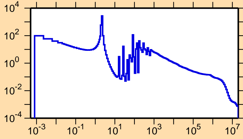
\sigma vs. E for ^{137}\text{La}(n,\gamma)
