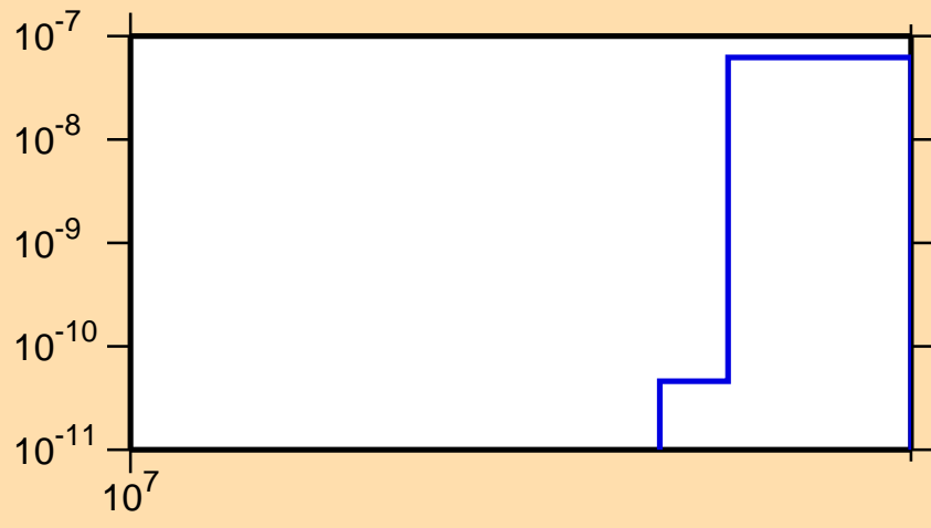
\sigma vs. E for ^{137}\text{La}(n,nt)
