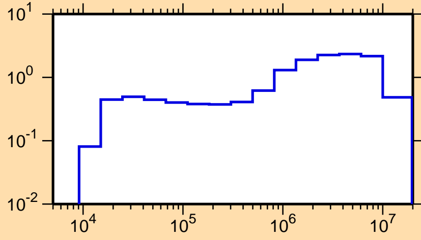
\sigma vs. E for ^{137}\text{La}(n,\text{inel.})
