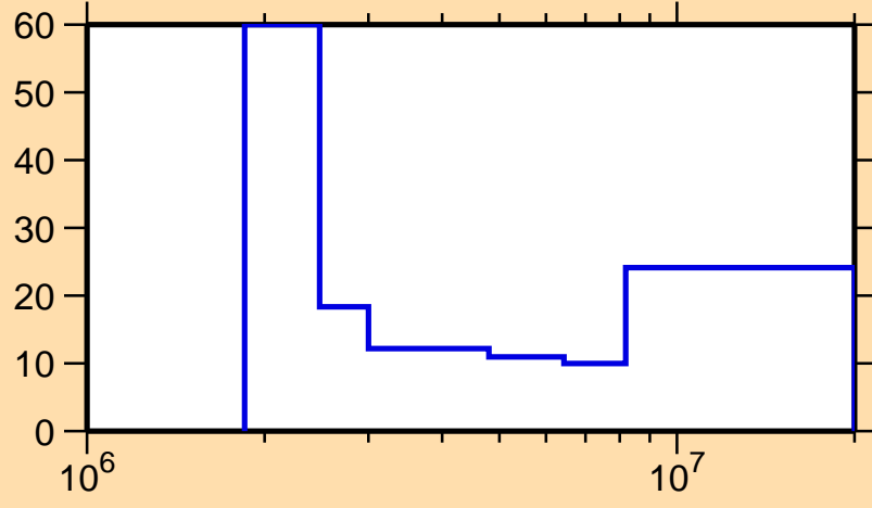
\Delta\sigma/\sigma vs. E for ^{137}\text{La}(n,n\text{cont.})
