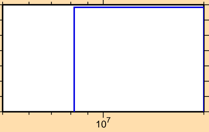
\sigma vs. E for ^{137}\text{La}(n,t)
