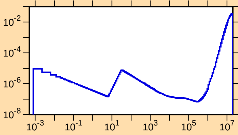
\sigma vs. E for ^{138}\text{La}(n,p)
