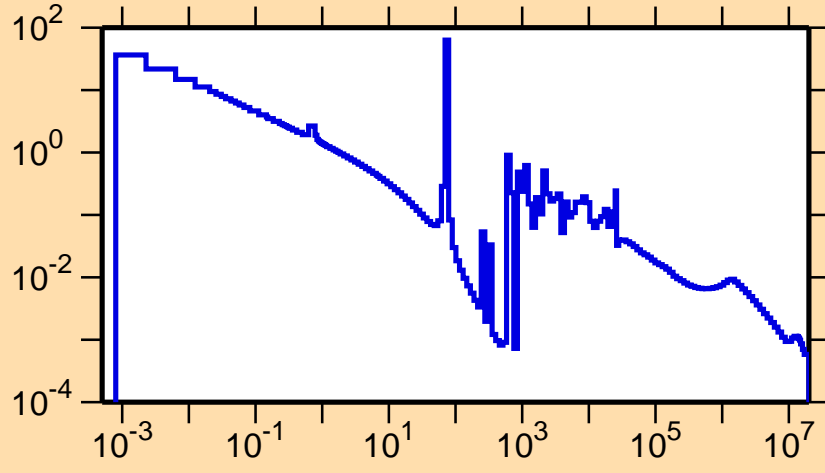
\sigma vs. E for ^{139}\text{La}(n,\gamma)
