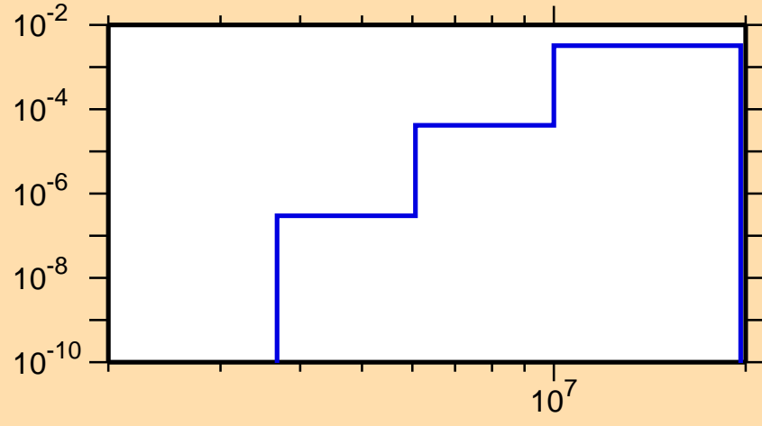
\sigma vs. E for ^{139}\text{La}(n,p)
