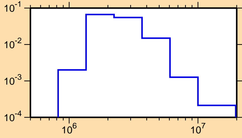
\sigma vs. E for ^{139}\text{La}(n,n_4)
