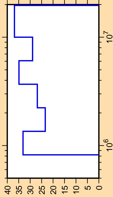
\Delta\sigma/\sigma vs. E for ^{139}\text{La}(n,n_4)
