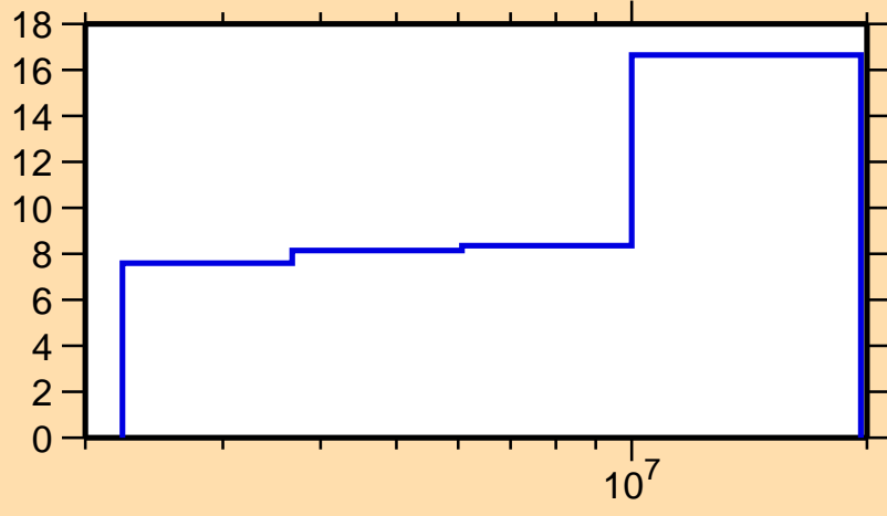
\Delta\sigma/\sigma vs. E for ^{139}\text{La}(n,n\text{cont.})
