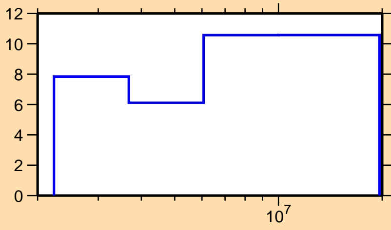
\Delta\sigma/\sigma vs. E for ^{139}\text{La}(n,el.)
