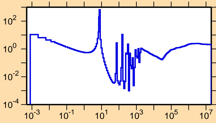
\sigma vs. E for ^{140}\text{La}(n,\text{nonel.})
