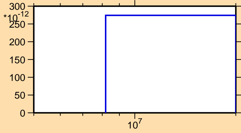
\sigma vs. E for ^{140}\text{La}(n,p\alpha)
