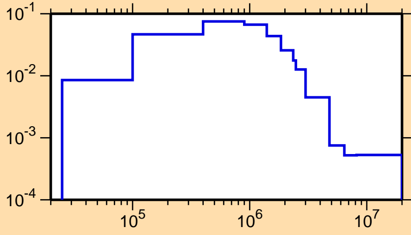
\sigma vs. E for ^{140}\text{La}(n,n_3)
