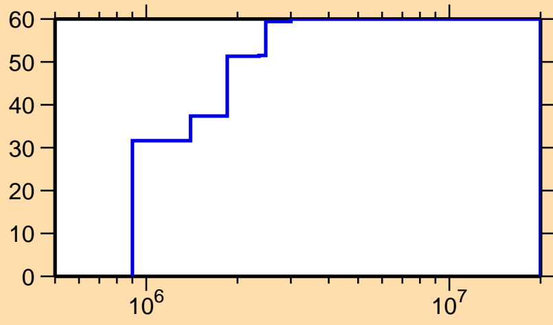
\Delta\sigma/\sigma vs. E for ^{140}\text{La}(n,n_1)
