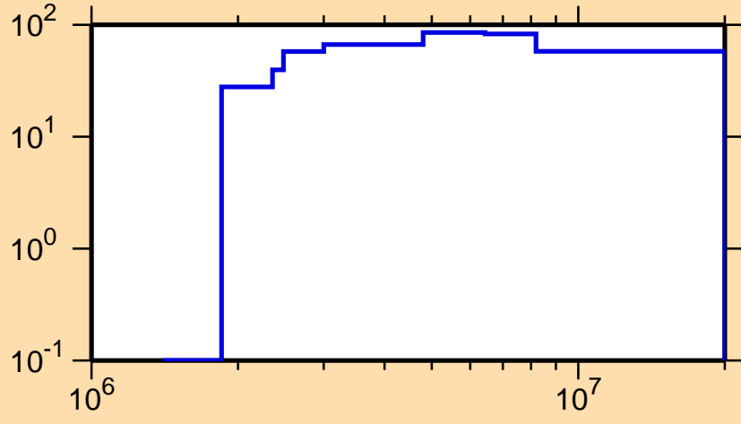
\Delta\sigma/\sigma vs. E for ^{140}\text{La}(n,p)
