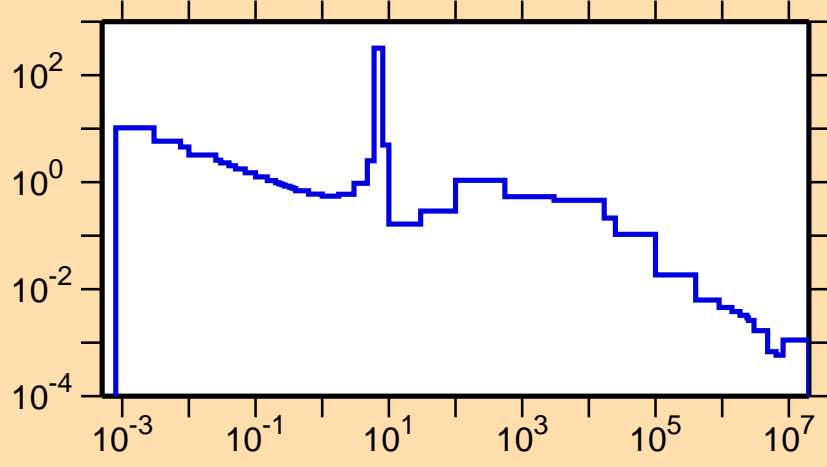
\sigma vs. E for ^{140}\text{La}(n,\gamma)
