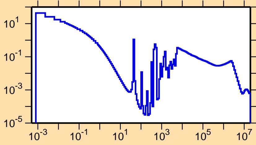
\sigma vs. E for ^{141}\text{La}(n,\gamma)
