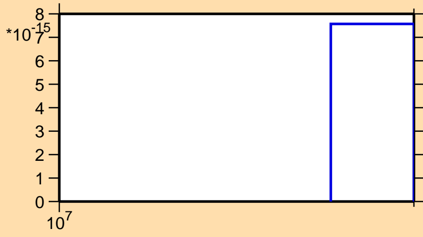
\sigma vs. E for ^{141}\text{La} (mt 42)
