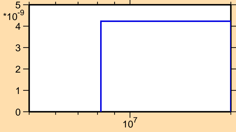
\sigma vs. E for ^{141}\text{La}(n,2n\alpha)
