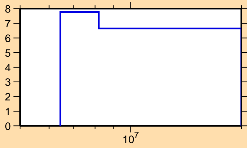
\Delta\sigma/\sigma vs. E for ^{141}\text{La}(n,\text{nonel.})
