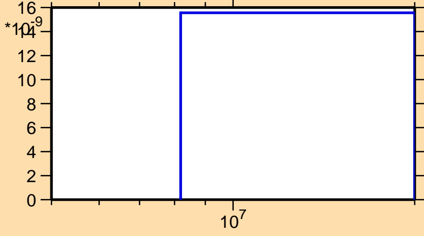
\sigma vs. E for ^{141}\text{La}(n,2np)
