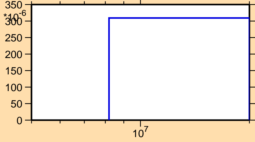
\sigma vs. E for ^{141}\text{La}(n,np)
