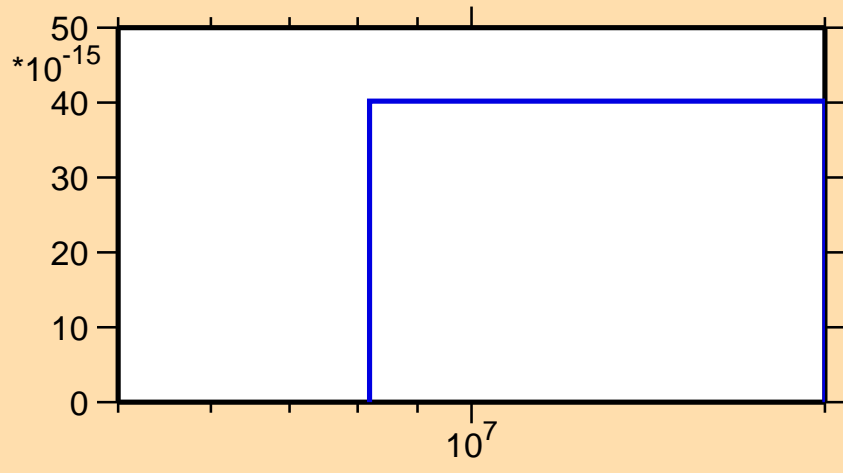
\sigma vs. E for ^{141}\text{La} (mt 11)
