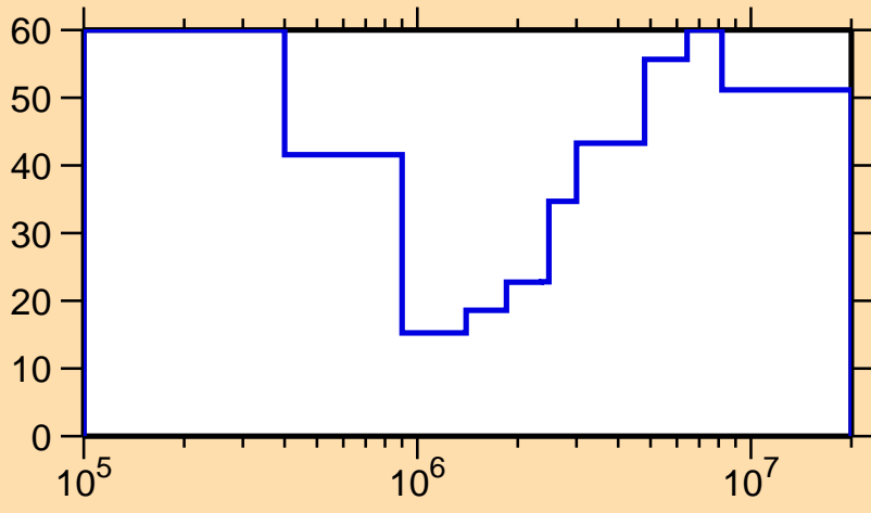
\Delta\sigma/\sigma vs. E for ^{141}\text{La}(n,n_1)
