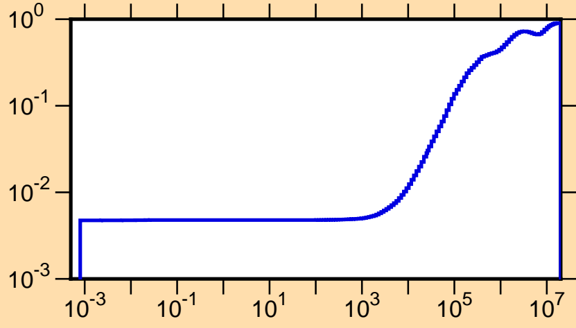
\mu vs. E for ^{142}\text{La}(\text{mt251})
