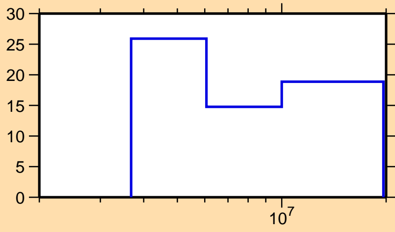
\Delta\sigma/\sigma vs. E for ^{142}\text{La}(n,2n)
