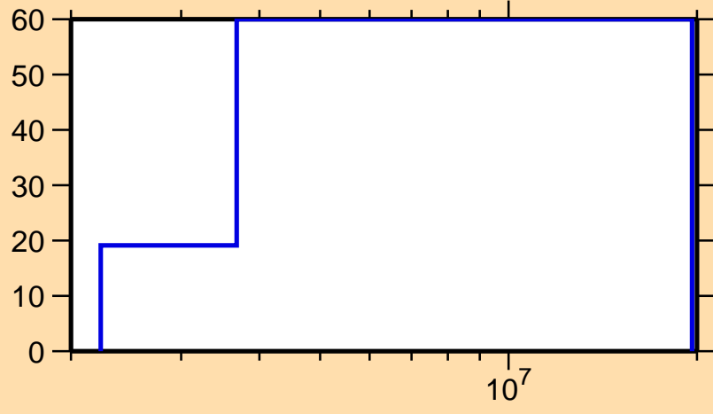
\Delta\sigma/\sigma vs. E for ^{142}\text{La}(n,p)
