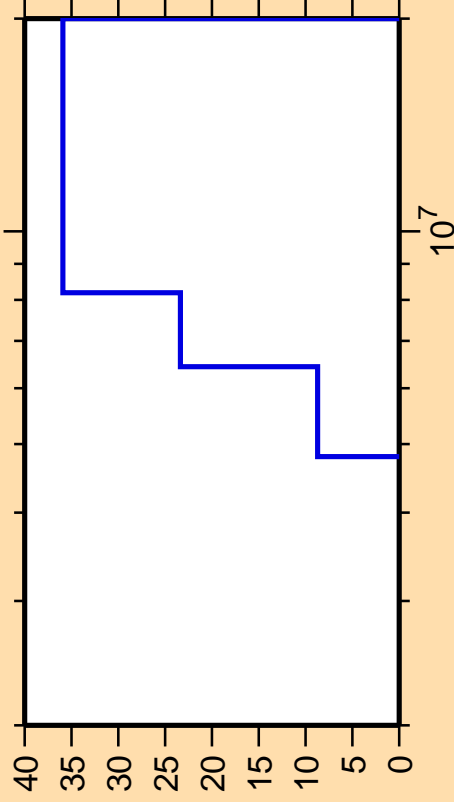
\Delta\sigma/\sigma vs. E for ^{142}\text{La}(n,n\text{cont.})
