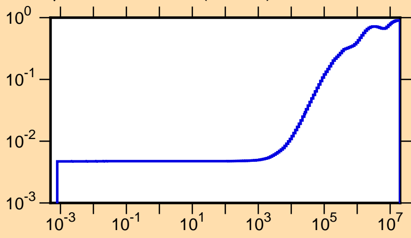
\mu vs. E for ^{143}\text{La}(\text{mt251})
