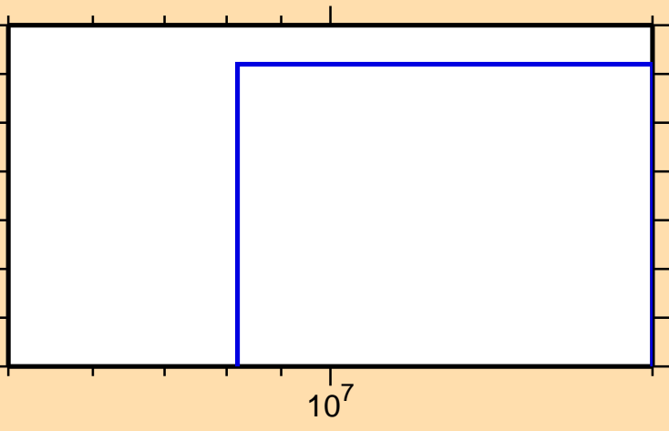
\sigma vs. E for ^{143}\text{La}(n,3n\alpha)
