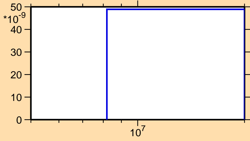
\sigma vs. E for ^{143}\text{La}(n,2n\alpha)
