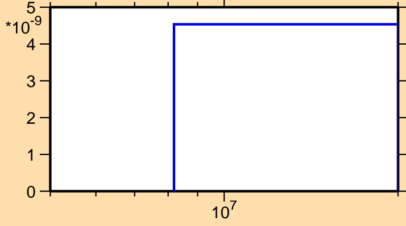
\sigma vs. E for ^{143}\text{La}(n,2np)
