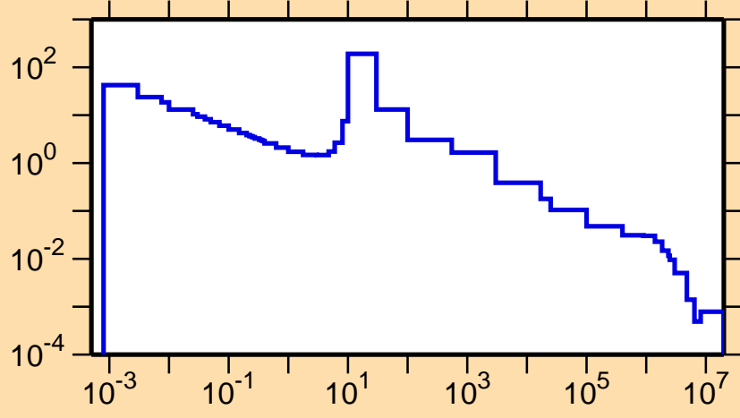
\sigma vs. E for ^{143}\text{La}(n,\gamma)
