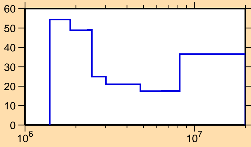
\Delta\sigma/\sigma vs. E for ^{143}\text{La}(n,n\text{cont.})
