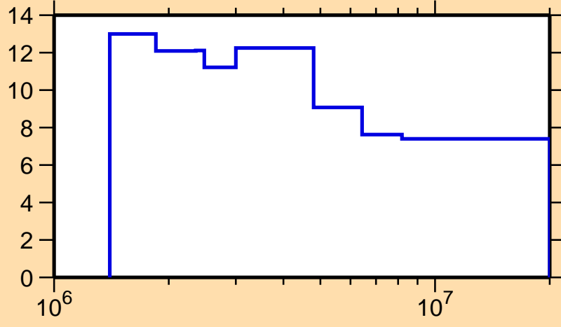
\Delta\sigma/\sigma vs. E for ^{143}\text{La}(n,n\text{onel.})
