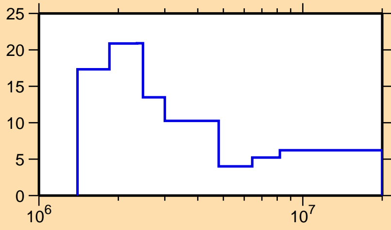
\Delta\sigma/\sigma vs. E for ^{143}\text{La}(n,\text{tot.})
