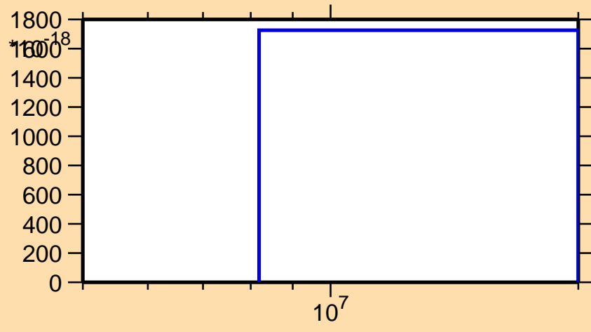
\sigma vs. E for ^{143}\text{La}(n,\text{He3})
