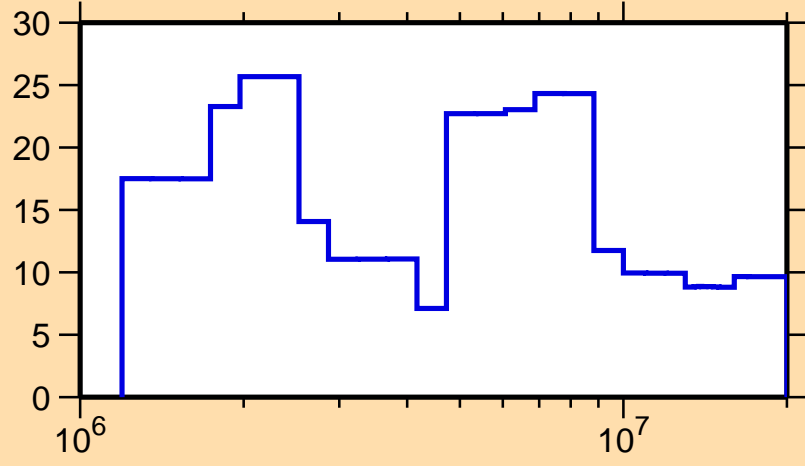
\Delta\sigma/\sigma vs. E for ^{144}\text{La}(n, el.)
