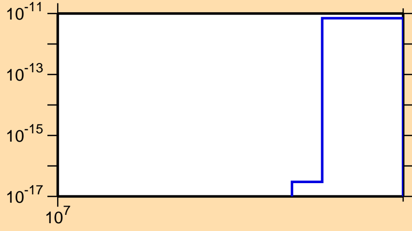
\sigma vs. E for ^{144}\text{La} (mt 11)
