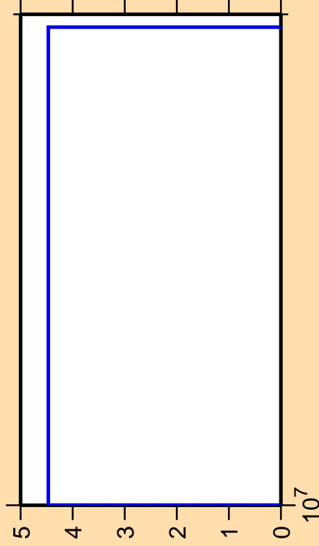
\Delta\sigma/\sigma vs. E for ^{144}\text{La}(n,3n\alpha)
