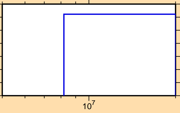
\sigma vs. E for ^{144}\text{La}(n,\text{nd})
