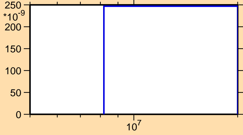
\sigma vs. E for ^{144}\text{La}(n,2n\alpha)
