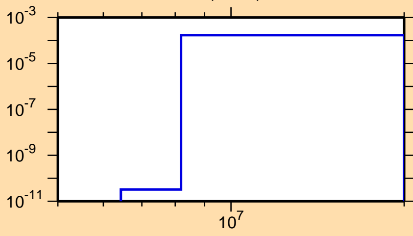
\sigma vs. E for ^{144}\text{La}(n,n\alpha)
