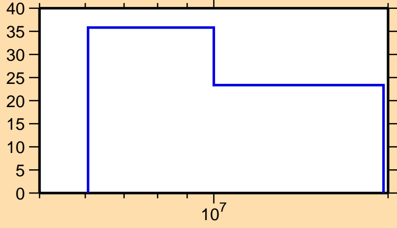
\Delta\sigma/\sigma vs. E for ^{145}\text{La}(n,el.)
