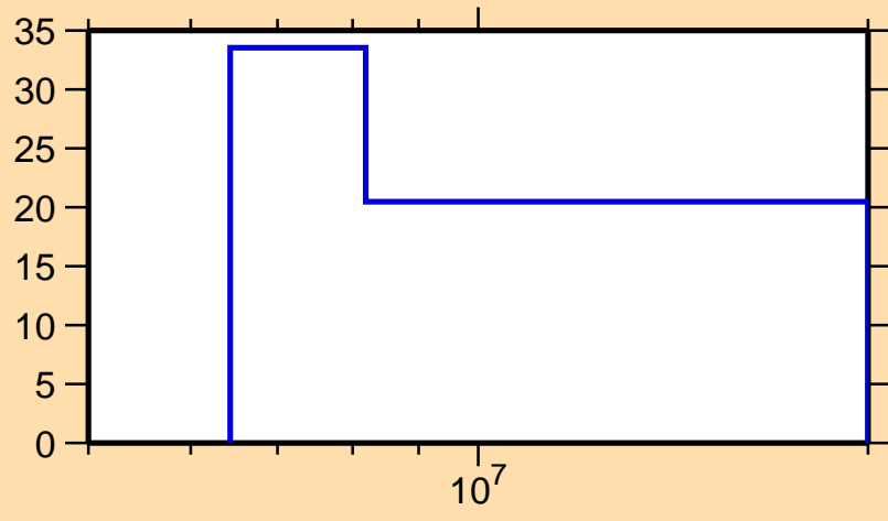
\Delta\sigma/\sigma vs. E for ^{145}\text{La}(n,el.)
