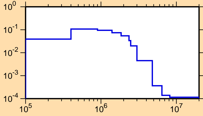
\sigma vs. E for ^{145}\text{La}(n,n_3)
