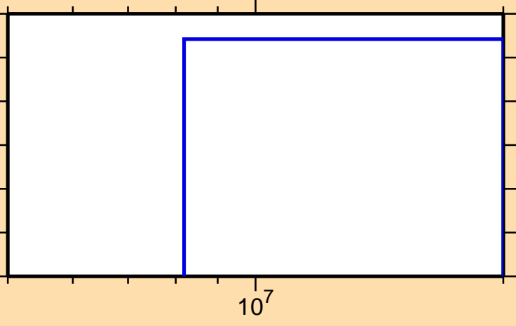
\sigma vs. E for ^{145}\text{La}(n,3n)
