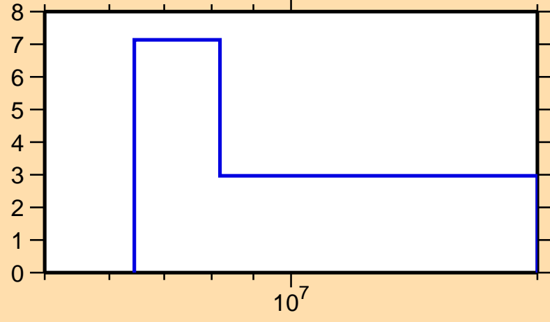
\Delta\sigma/\sigma vs. E for ^{145}\text{La}(n,\text{nonel.})
