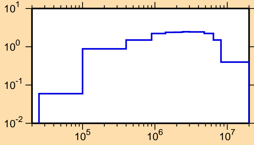
\sigma vs. E for ^{145}\text{La}(n,\text{inel.})
