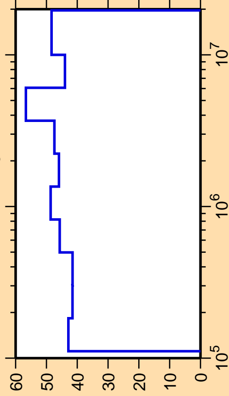
\Delta\sigma/\sigma vs. E for ^{146}\text{La}(n,n_3)
