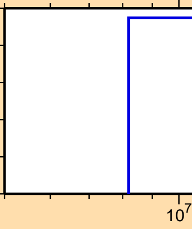
\sigma vs. E for ^{146}\text{La}(n,\text{nd})
