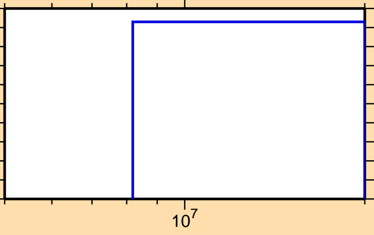
\sigma vs. E for ^{146}\text{La}(n,nt)
