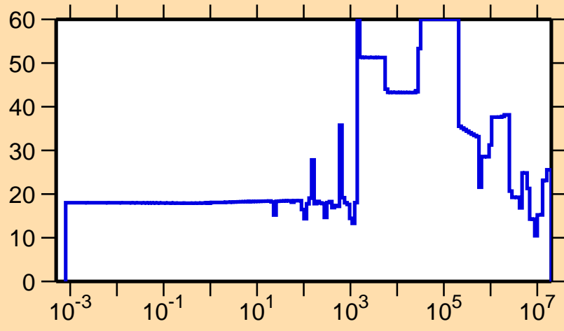
\Delta\sigma/\sigma vs. E for ^{146}\text{La}(n,\text{el.})
